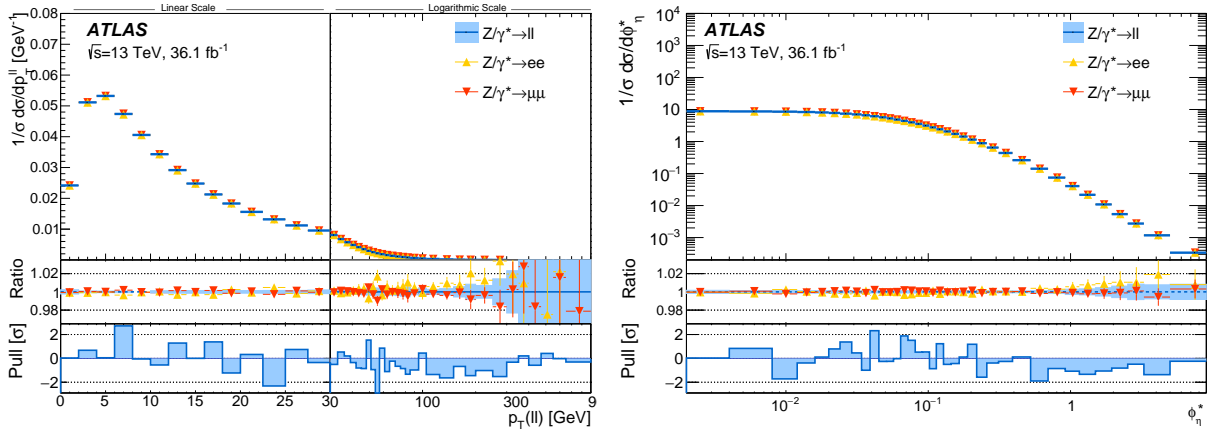
Figure 4: The measured normalized cross section as a function of p_T^{\ell\ell} (left) and \phi_n^* (right) for the electron and muon channels and the combined result as well as their ratio together with the total uncertainties, shown as a blue band. The pull distribution between the electron and muon channels, defined as the difference between the two channels divided by the combined uncorrelated uncertainty, is also shown. The p_T^{\ell\ell} distribution is split into linear and logarithmic scales at 30 GeV.
