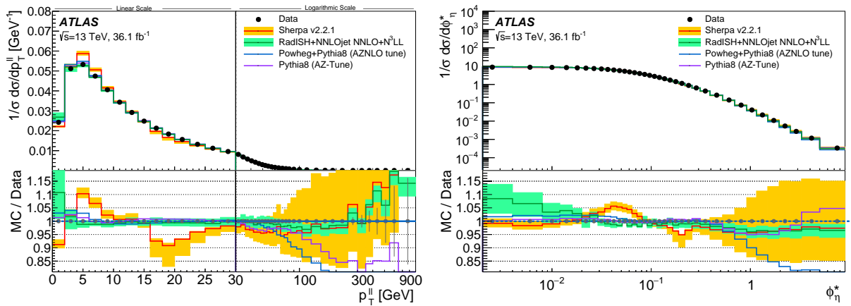
Figure 5: Comparison of the normalized p_T^{\ell\ell} (left) and \phi_\eta^* (right) distributions predicted by different computations: PYTHIA8 with the AZ tune, POWHEG+PYTHIA8 with the AZNLO tune, SHERPA v2.2.1 and RADISH with the Born level combined measurement. The uncertainties of the measurement are shown as vertical bars and uncertainties of the SHERPA and RADISH predictions are indicated by the coloured bands.
