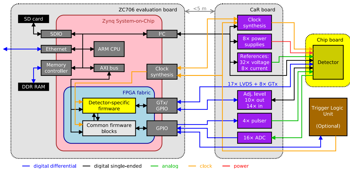
Figure 2: Simplified schematics of the Caribou hardware architecture.
