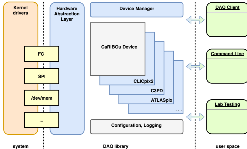
Figure 3: Peary DAQ software architecture.
