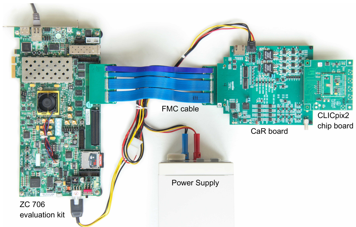
Figure 1: A complete Caribou DAQ setup.
