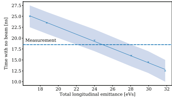
Fig. 8: Simulated duration of the particle-free region vs. total longitudinal emittance. The uncertainty in determining this time ( \pm 2.5 ns, light blue area) is dominated by the shape of the projections of the simulated bunch distribution.
