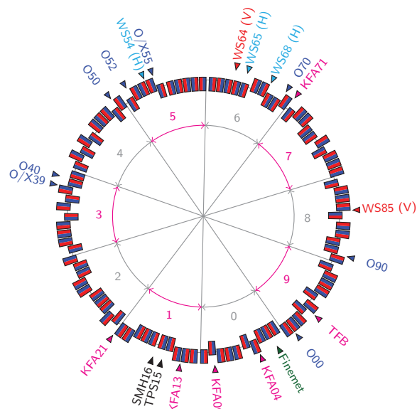
Fig. 2: Layout of the PS ring including the combined-function main magnets (red and blue rectangles for the focusing and defocusing parts, respectively, where the radial offset between the rectangles accounts for the four different magnet types [24]) and the location of the key elements for MTE: sextupoles and octupoles (element names starting with X or O), fast dipoles for beam extraction (element names starting with K), magnetic (SMH16) and dummy (TPS15) septa, and wire scanners (element names starting with W) for the measurement of the transverse beam distributions. The position of the Finemet ® cavity [25] used for the generation of the barrier bucket is also indicated.
