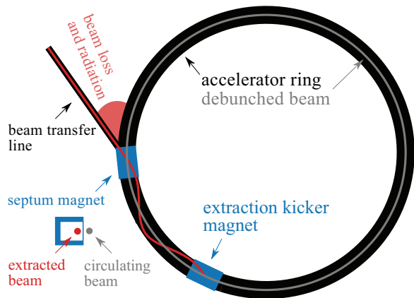
Fig. 1: Sketch of the principle of beam extraction with the beam losses induced by the continuous longitudinal distribution. The rise time of the kickers is of the order of 390 ns, referring to the time needed to increase the kicker strength from 5% to 95% of the nominal value (one PS turn corresponds to 2.1 \mu s).
