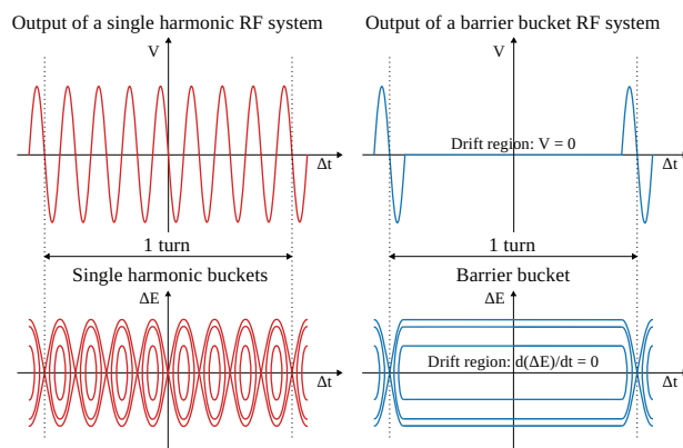
Fig. 3: Comparison of a single-harmonic waveform and corresponding longitudinal phase space (left) and a barrier bucket waveform and corresponding phase space (right).
