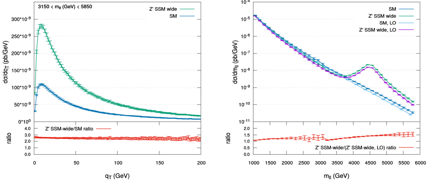
Fig. 1. (a) Distribution in the transverse momentum of the di-lepton system calculated at NNLL for the SM (dark blue) and the SSM wide (green) scenario with M_{Z'} = 4.5 TeV. We select the invariant mass region relevant for the Z' boson search 3150 \text{ GeV} \leq M_{II} \leq 5850 \text{ GeV} . The lower plot shows the ratio of the SSM wide Z' boson q_T spectrum to the SM one at NNLL. The bars indicate MC errors. (b) Di-lepton invariant mass ( M_{II} ) distribution for the SM at LO (light blue) and NNLL (dark blue) and the SSM wide scenario at LO (purple) and at NNLL (green) with M_{Z'} = 4.5 TeV. The lower plot shows the ratio between the NNLL and LO invariant mass spectrum for the SSM wide case. The bars indicate MC errors.
