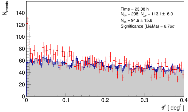
(a) \theta^2 plot.
