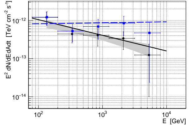
Figure 2: VHE SED from 2WHSP J073326.7+515354. The black markers and line represent the observed SED spectral data and fit. The intrinsic SED after correcting for the EBL absorption assuming the model from Dominguez et al. (2011) is represented in blue. The shaded area represents the uncertainty obtained from a forward folding method ( Mizobuchi et al. 2005 ).
