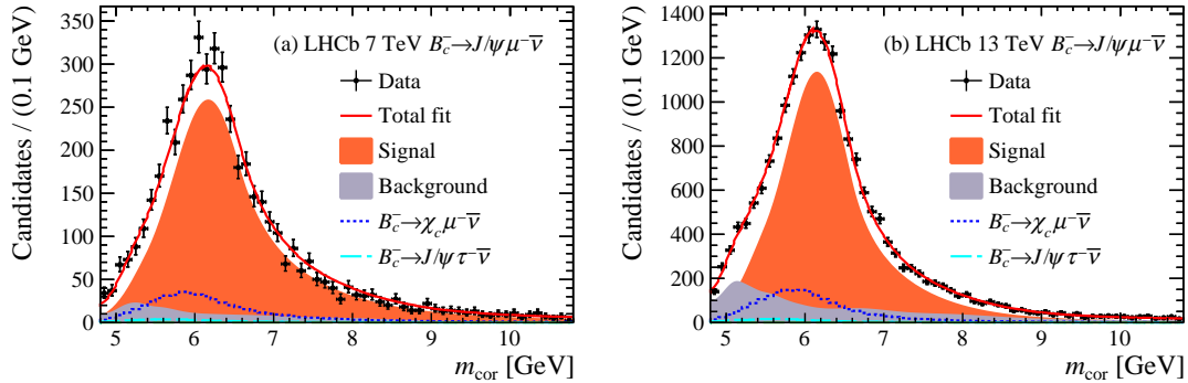
Figure 2: Fitted m_{\text{cor}} distributions in (a) 7 TeV and (b) 13 TeV samples. The signal and the backgrounds are shown as the dark (orange) and lighter (gray) areas. The dashed (cyan) curves show the B_c^- \rightarrow J/\psi \tau^- \nu_\tau components, while the dotted (blue) curves show the B_c^- \rightarrow \chi_{c0,1,2} \mu^- \bar{\nu} components. The B_c^- \rightarrow \psi(2S) \mu^- \bar{\nu} contribution is also in the fit but is too small to be seen. The total fit is shown by the solid (red) curve.
