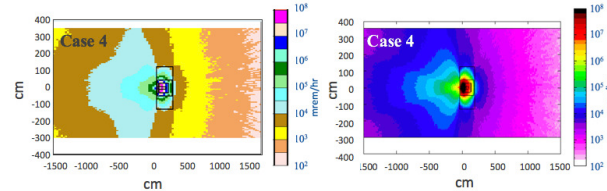
Figure 4: FLUKA and MARS15 Case 4 results. The two code results agree on the ambient dose equivalent rates due to prompt radiation at 2 mA, 185 MeV, Scenario A .
