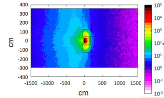
Figure 7: FLUKA Case 4 residual radiation results. 20 mrem/hr is considered a good practice limit for access the zone surrounding the beam absorber.
