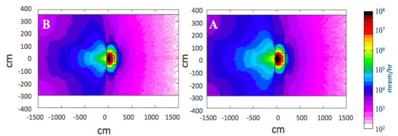
Figure 5: FLUKA Case 4 results comparison between beam pulsed Scenario A (right) and Scenario B (left) at 185 MeV. Restriction to access still applied, based on Scenario B results. However, access restricted to authorized personnel can be allowed during beam-on operation if a rigid barrier with locked gates is installed at approximately 15 m downstream the beam absorber.
