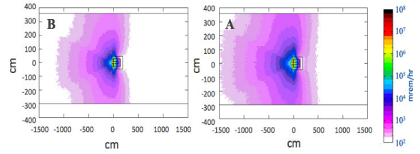
Figure 6: FLUKA Case 1 35 MeV results for Scenario A (right) and for Scenario B (left).
