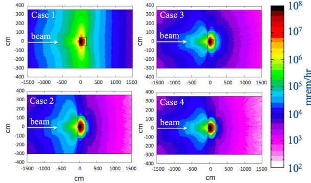
Figure 3: FLUKA results comparison between the ambient dose equivalent rates due to prompt radiation at 2 mA, 185 MeV and Scenario A for the four shielding cases.
