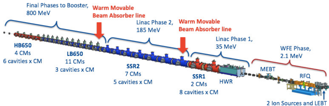
Figure 1: 3D Model of the ~215 m long PIP-II accelerator from the two H - ions sources (right) to the HB650 section (left). Beam Commissioning Phases are shown as well as the proposed Warm Movable Beam Absorber locations: at the first SSR2 CM (to allow the Linac Phase 1 Beam Commissioning) and at the first LB650 CM (to allow the Linac Phase 2 Beam Commissioning).
