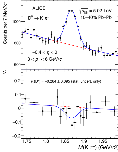
Figure 1: (color online) Illustration of the D^0 meson v_1 extraction procedure via a simultaneous fit to the candidate invariant mass distribution (upper panel) and v_1 (lower panel) for 3 < p_T < 6 GeV/c and -0.4 < \eta < 0 in the 10–40% centrality interval. The blue solid lines correspond to the combined signal and background fit functions, while the red dashed lines represent the background contribution.
