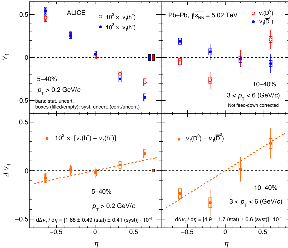
Figure 2: (color online) Upper left: v_1 of positively (red) and negatively (blue) charged hadrons for the 5–40% centrality interval. Upper right: v_1 of D^0 (red) and \bar{D}^0 (blue) for the 10–40% centrality interval. Lower left and right: \Delta v_1(h) = v_1(h^+) - v_1(h^-) and \Delta v_1(D) = v_1(D^0) - v_1(\bar{D}^0) , respectively. Dashed lines represent fits with a linear function.
