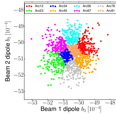
Figure 1: Illustration of the clustering to sort according to the b_3 component in both beams.
