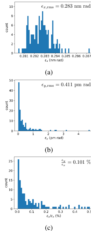
Figure 4: Distribution of (a) horizontal emittance, (b) vertical emittance, and (c) coupling ratio of the corrected Z lattices. The errors introduced are summarized in Table 2.
