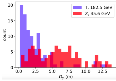
Figure 2: Distribution of the maximum vertical dispersion from introducing quadrupoles vertical offsets of 2 \mu\text{m} .
