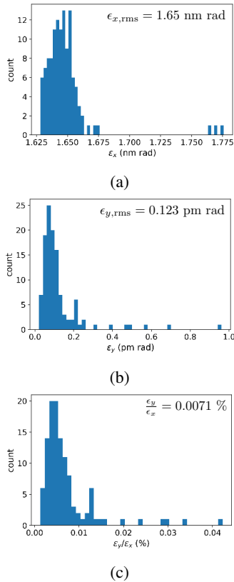
Figure 3: Distribution of (a) horizontal emittance, (b) vertical emittance, and (c) coupling ratio of the corrected ttbar lattices. The errors introduced are summarized in Table 2.
