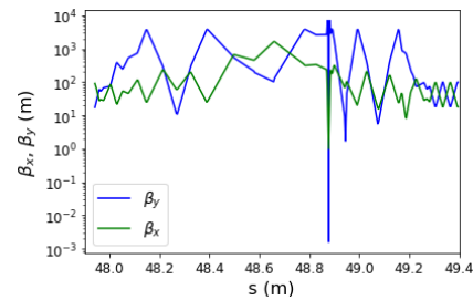
Figure 1: Beta functions near the IP of the 182.5 GeV lattice.
