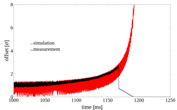
Figure 2: Measured (black) and simulated (red) orbit offset during ramp with CCs at 1 MV. The beam is excited by the effective phase slip of the CC excitation due to the beam revolution frequency changing as an effect of the beam energy increase.
