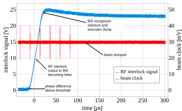
Figure 1: Test of the hardware interlock on phase difference between CCs and main beam RF. As the phase difference reaches its threshold, the RF interlock signal (blue) to the beam interlock system (BIS) changes to high making the BIS trigger a beam dump. The beam clock (one "spike" per turn) is shown in red.
