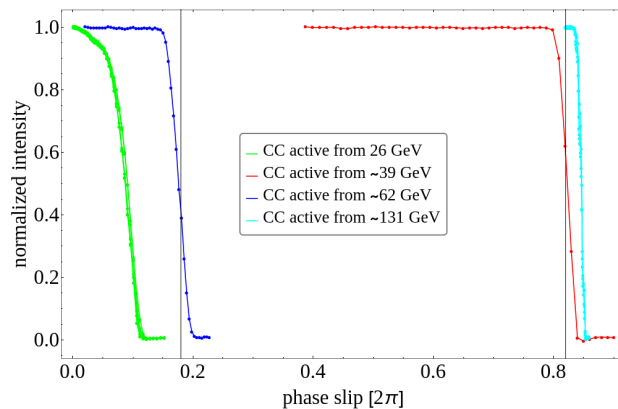
Figure 4: Energy scan of the fast losses during ramp, with the normalized beam intensity versus the phase slip. The black vertical lines indicate the vertical tune, as well as its complement. The beam intensity resolution is 5 ms.
