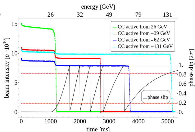
Figure 3: Change of beam intensity during the energy ramp, when activating the crab cavities at different energy levels. The starting time corresponds to the moment of injection. The energy ramps start at 1000 ms. The green, red, blue and cyan curves show the beam intensity during the different measurements. The black curve shows the phase slip as it changes throughout the ramp, and the dashed red lines indicate when it crosses the tune and its complement.
