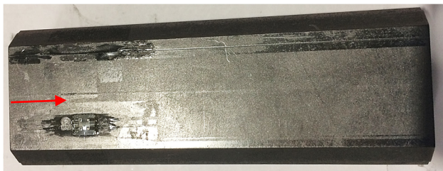
Figure 3: Visual inspection of most loaded MoGr block (#2). Red arrow indicates beam-induced mark. The other visible horizontal signs are optical fibre grooves and the glue used to fix them. Strain gauges are also visible.
