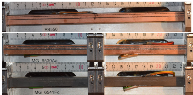
Figure 7: Visual inspection of Multimat targets: Cu-coated graphite (top), Cu-coated MoGr (center) and Mo-coated MoGr (bottom).
