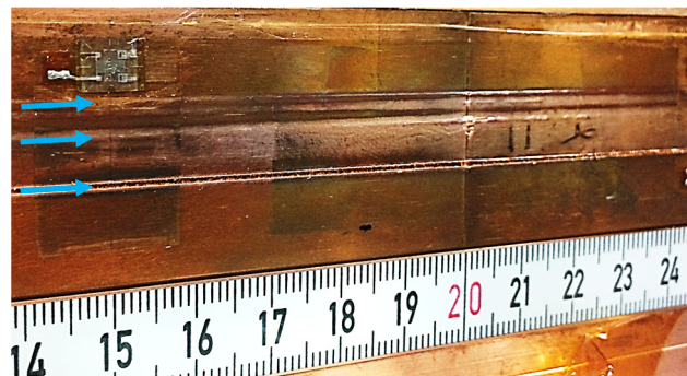
Figure 5: Visual inspection of CuCD jaw. Effects of the grazing impacts are indicated by the blue arrows.
