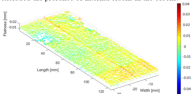
Figure 4: Flatness measurement of MoGr block #2.
