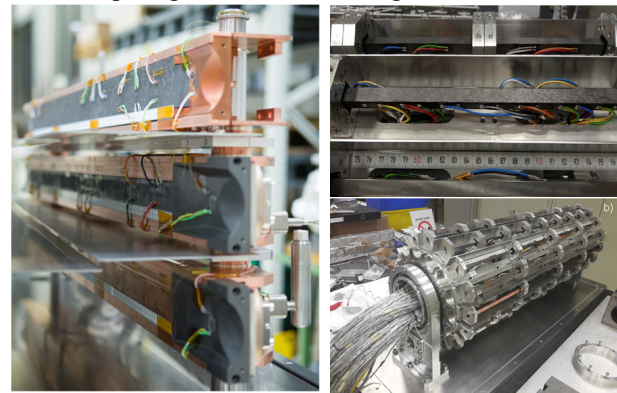
Figure 2: Configuration of Jaws, with, from top to bottom, CFC, MoGr and CuCD jaws (left) and Multimat (right).
