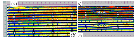
Figure 9: UT of MoGr (a) and CuCD (b) brazed interfaces, over different lengths: 200-550 mm (left) and 490-840 mm (right).
