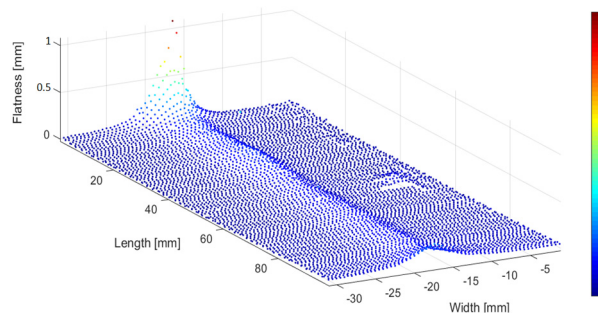
Figure 6: Flatness measurement of CuCD block #5, showing the area affected by the most severe impact, a factor of 3 above the ABD accident scenario.
