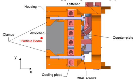
Figure 1: HL-LHC collimator jaw section view.
