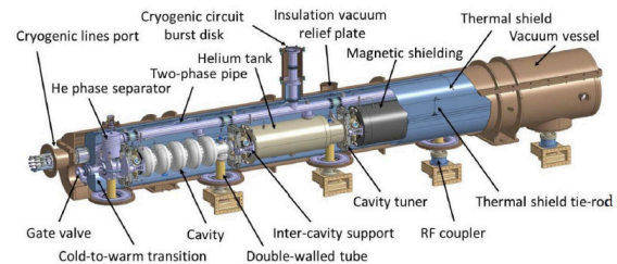
Figure 4: General assembly view of the SPL cryomodule considered to be adapted for PERLE.
