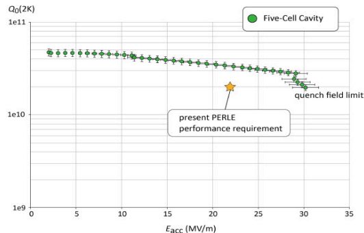
Figure 3: Vertical test result of the 5-cell 801.6 MHz Niobium cavity. The yellow star indicates the edge of the performances considered for PERLE operation.
