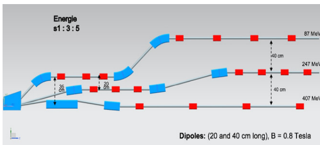
Figure 2: PERLE spreader design and matching to three circulating arcs.
