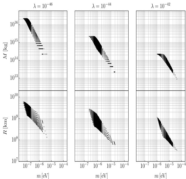
FIG. 1: Total mass M and radius R of the boson star subject to the Higgs portal vs. particle mass m for which \beta = 10^{-2} , \delta\omega/\omega \geq 10^{-18} , the frequency of collisions between the ADM boson star and the detector is f \geq 1 \text{ yr}^{-1} , and the self-coupling of the ADM is \lambda = 10^{-46} (left panel), \lambda = 10^{-44} (middle panel), and \lambda = 10^{-42} (right panel). Notice that this value of \beta is excluded from BBN constraints if the ADM is assumed to have formed before BBN.
