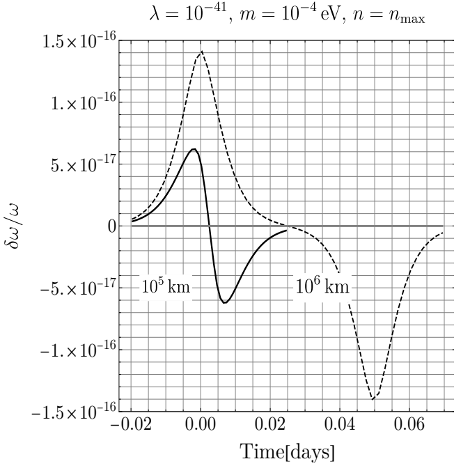
FIG. 10: The relative induced fractional frequency shift \delta\omega/\omega|_{\text{rel}} vs. time as two synchronized optical atomic clocks pass through a boson star subject to the photon portal. The boson star is taken to have parameters \lambda = 10^{-41} , m = 10^{-4} eV, n = n_{\text{max}} , and g = 10^{-10} GeV ^{-2} which results in M \sim \times 10^{14} kg, R_{99} \sim 10^5 km, and f \sim 10^{-5} yr ^{-1} . The minimum time here is taken to be when the edge of the boson star starts to pass through the first clock, while the maximum time is taken to be the time at which the boson star fully passes through the second clock. The dashed line corresponds to a distance of 10^6 km between the detectors while the thick line corresponds to a distance of 10^5 km. The filled in region corresponds to |\delta\omega/\omega|_{\text{rel}} \leq 10^{-20}
