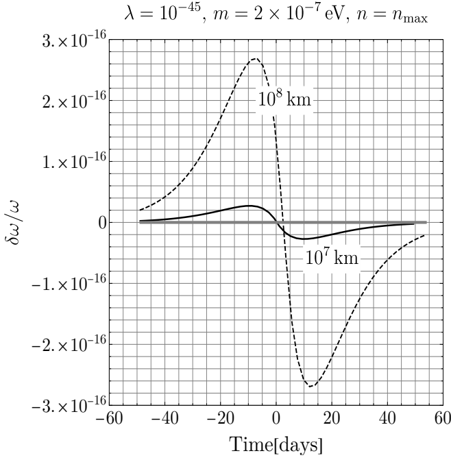
FIG. 5: The relative induced fractional frequency shift \delta\omega/\omega|_{\text{rel}} vs. time as two synchronized microwave atomic clocks pass through a boson star. The boson star is taken to have parameters \lambda = 10^{-45} , m = 2 \times 10^{-7} eV, n = n_{\text{max}} , and \beta = 10^{-2} which results in M \sim 10^{16} kg, R_{99} \sim 10^9 km, and f \sim 2 \text{ yr}^{-1} . The minimum time here is taken to be when the edge of the boson star starts to pass through the first clock, while the maximum time is taken to be the time at which the boson star fully passes through the second clock. The dashed line corresponds to a distance of 10^8 km between the detectors while the thick line corresponds to a distance of 10^7 km. The filled in region corresponds to |\delta\omega/\omega|_{\text{rel}} \leq 10^{-18} . Notice that this value of \beta is excluded from BBN constraints if the ADM is assumed to have formed before BBN.
