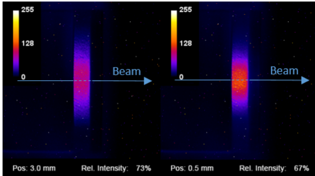
Figure 2: ChDR light recorded on the camera for a beam to dielectric distance of 3 mm (left) and 0.5 mm (right).
