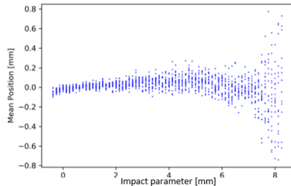
Figure 4: Vertical position of the beam during the impact parameter scan.
