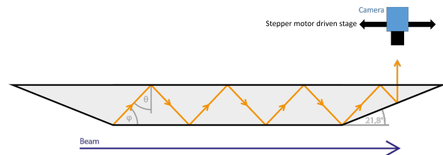
Figure 1: View from the top. The radiation produced all along the surface of the radiator is emitted at the characteristic Cherenkov angle and reflected inside the radiator before extraction to a camera.
