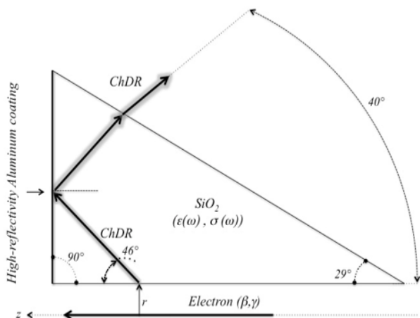
Figure 5: Radiator installed at ATF2.
