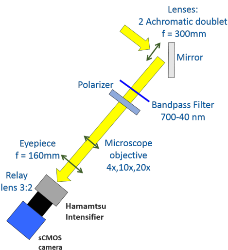
Figure 7: New optical line at ATF2. The yellow arrows represent the ChDR light path.
