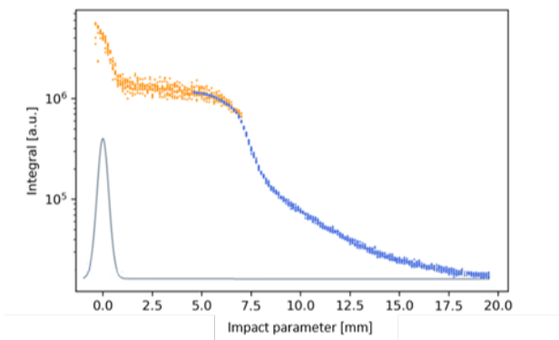
Figure 3: Impact parameter scan against total intensity of ChDR. The approximate beam profile is shown in grey.
