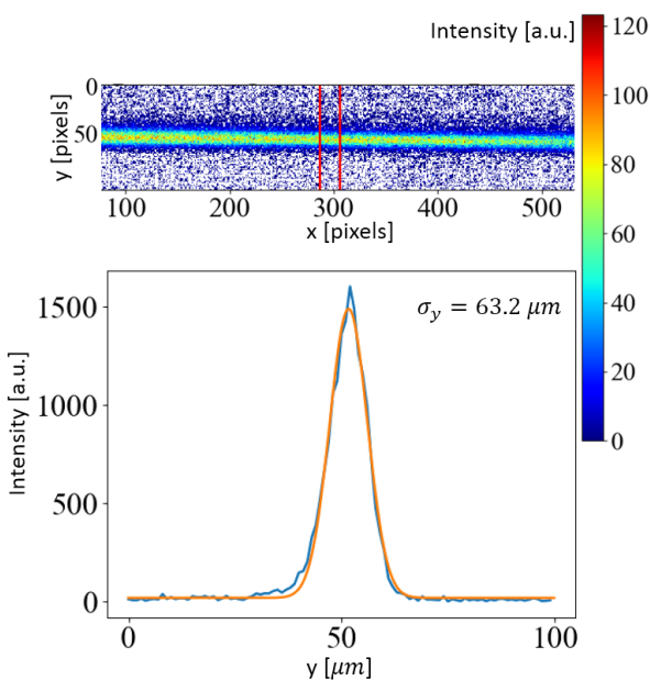
Figure 6: Diffraction Cherenkov 2D image and profile.
