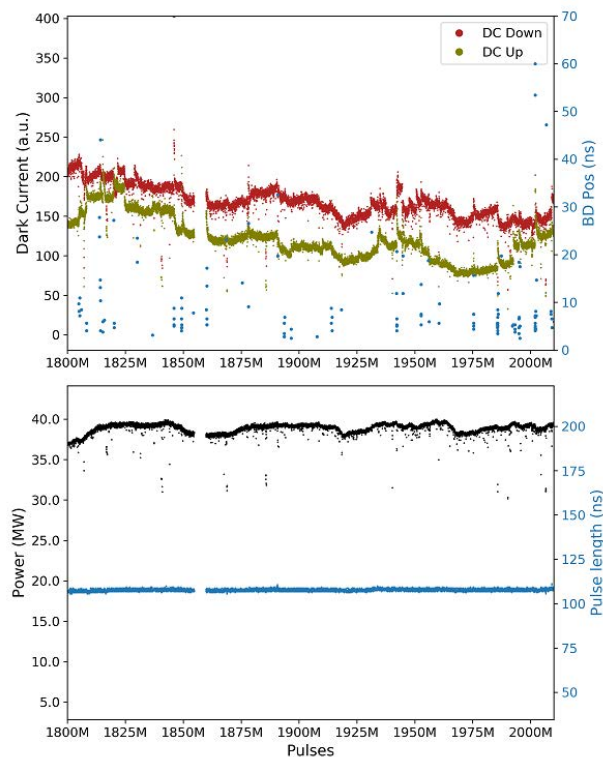
Figure 3: Fragment of conditioning of a TD24 tested in Xbox 3. The graph in the top shows the upstream and downstream dark currents measured, together with the breakdown positioning. The one in the bottom shows the power and the pulse length of the RF pulses.
