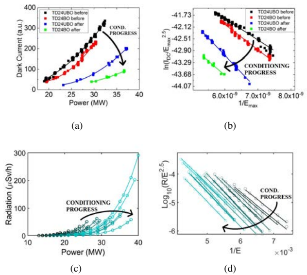
Figure 5: Power scans for two TD24 tested in Xbox 3: Dark current as a function of power (a), and Fowler-Nordheim plot for the same data (b). Power scans for a TD26CC tested in Xbox 2: Radiation as a function of power (c), and Fowler-Nordheim plot for the same data (d).
