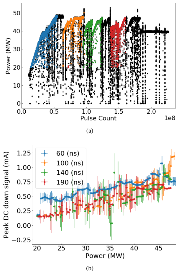
Figure 2: (a) RF power conditioning plot of the T24PSIN2 at Xbox 2, marking the different pulse length sectors. (b) Dark current versus RF power for different pulse lengths.
