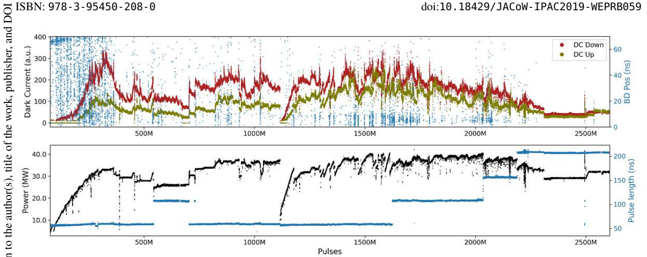
Figure 4: Full conditioning of a TD24 tested in Xbox 3. The graph in the top shows the upstream and downstream dark currents measured, together with the breakdown positioning. The one in the bottom shows the power and the pulse length.
