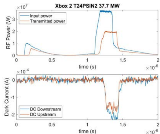
Figure 1: Example of traces measured at Xbox 2.
