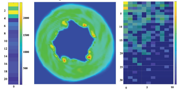
Figure 4: Polar Fourier decomposition of uniform and distorted beams: real part of coefficients P_{k0} for a uniform beam (left), the distorted beam image (middle), coefficients P_{km} for the distorted beam (right).
