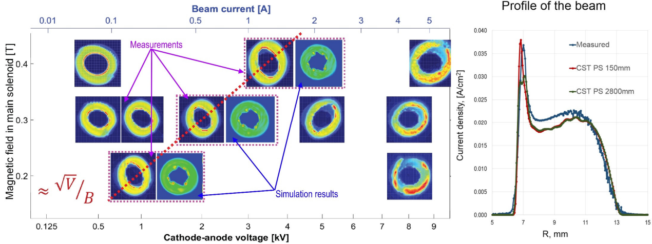
Figure 1: Measured and calculated profiles of the hollow beam depending on magnetic field in main solenoid and current of the beam (left), comparison of measured and simulated profiles (right).
