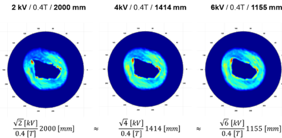
Figure 3: Examples of profiles with tilted injection.
