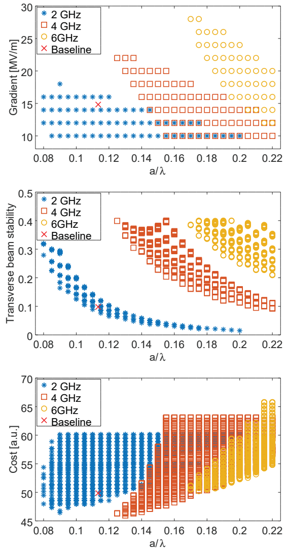
Figure 3: Results from the parameter scan. The plots show structures with different iris apertures and gradients (top), margins of transverse beam stability (middle) and costs (bottom).
