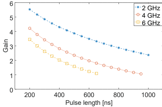
Figure 2: Gains for different pulse lengths of the compressed double-pulse for three different RF frequencies.
