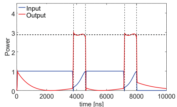
Figure 1: Example of pulse compressor input and output power signals. In this case a 2 GHz 8 \mu s klystron pulse is compressed to two 800 ns long pulses with a gain factor of 2.9.
