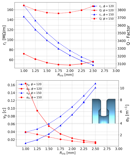
Figure 3: Plots of the shunt impedance and Q-factor (top), group velocity and attenuation factor (bottom) of the reentrant double bend geometry as a function of the iris aperture.
