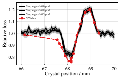
Figure 4: Relative beam loss measured on the BLMs next to the ES as a function of the crystal position when aligned to the beam in VR.
