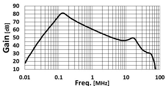
Figure 9: Cell Transfer Function.
