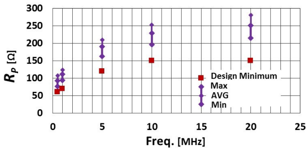
Figure 4: MA Cores Loss Resistance R_p .
