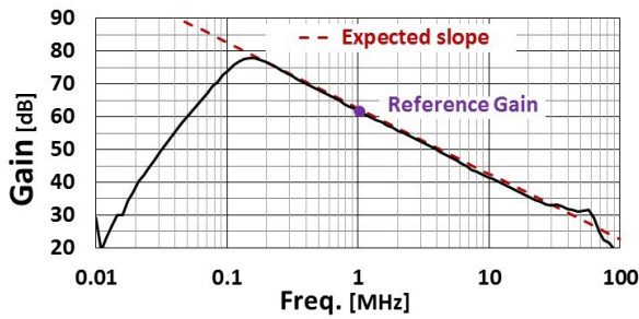
Figure 7: Power Amplifier Frequency Response.
