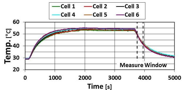
Figure 6: Thermal Transient for the Evaluation of the Water Sharing among Cells in one Cavity.
