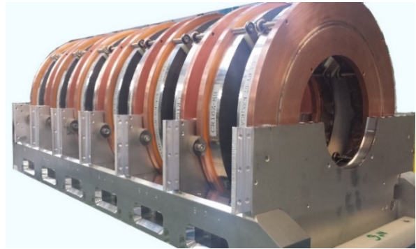
Figure 5: Cavity Shroud with MA Cores and Cooling Rings.
