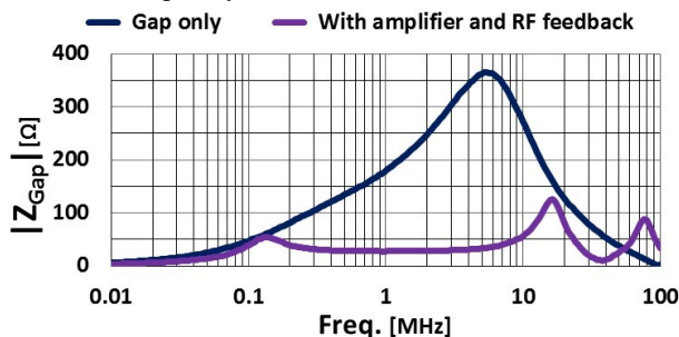
Figure 8: Cell Gap Impedance.
