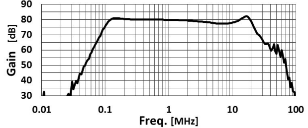
Figure 10: Linearized 6-Cell Cavity Transfer Function.
