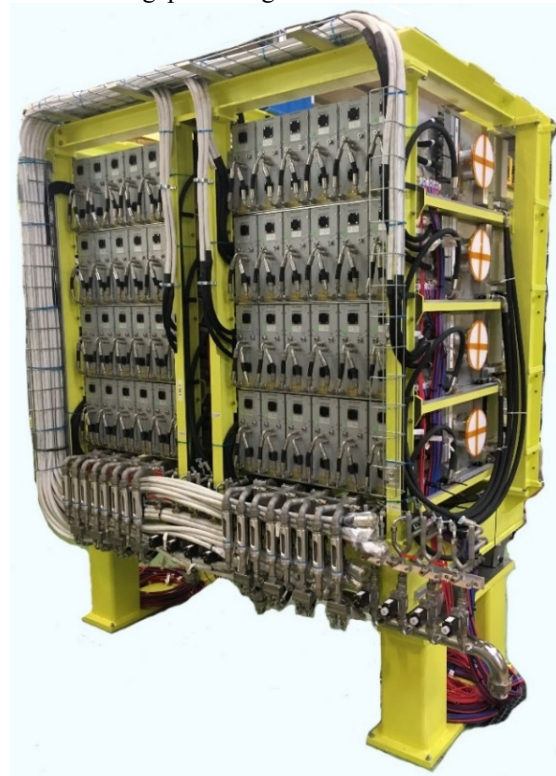
Figure 2: Cavities grouping for one PSB Straight Section.
