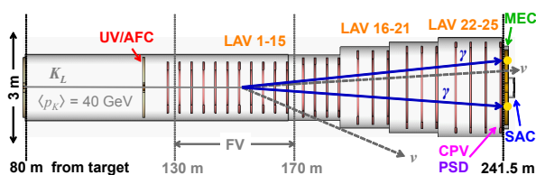
Figure 3: Layout of the detectors for KLEVER.
