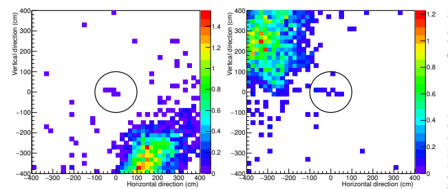
Figure 4: Rate per bin (MHz) for muons with P > 1 \text{ GeV}/c passing through the UV, (left) for \mu^+ and (right) for \mu^- . The large muon populations shown move outward and away from the downstream detector planes.
