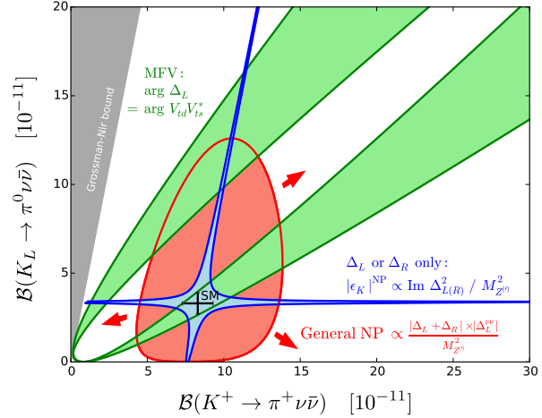
Figure 1: SM prediction for \text{BR}(K \rightarrow \pi \nu \bar{\nu}) with new physics scenarios overlaid, from [1]: CKM-like models with minimal flavour violation (green), models with flavour-violating interactions in which left-handed or right-handed couplings dominate (blue) and more general models (e.g., Randall-Sundrum, red).
