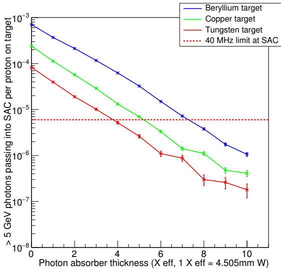
Figure 5: Rate of photons with E > 5 GeV per POT for varying thickness of photon absorber, for Be / Cu / W targets.
