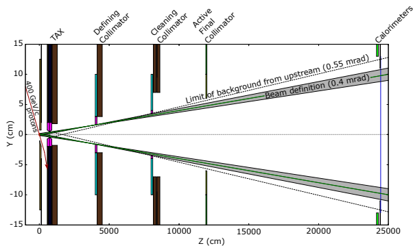
Figure 2: Layout of the K12 beamline for KLEVER, with the four-collimator system for selecting the neutral beam.
