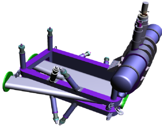
Figure 3: Cryostat and vacuum chamber of the branching dipole. Due to the opening for the chamber the coil casing supports have to be inclined to be able to cope with the magnetic forces.
