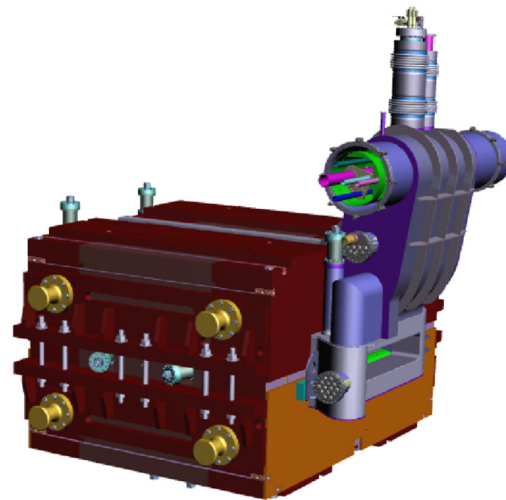
Figure 2: Outer shape of the dipole. One clearly sees the warm iron and the embedded cryostat. The big turret is due to the DN400 flange for the standardized cryogenic and electrical interfaces.
