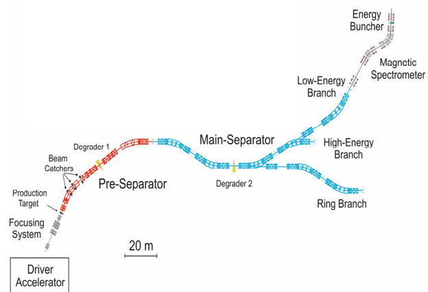
Figure 1: Magnetic layout of Super-FRS.
