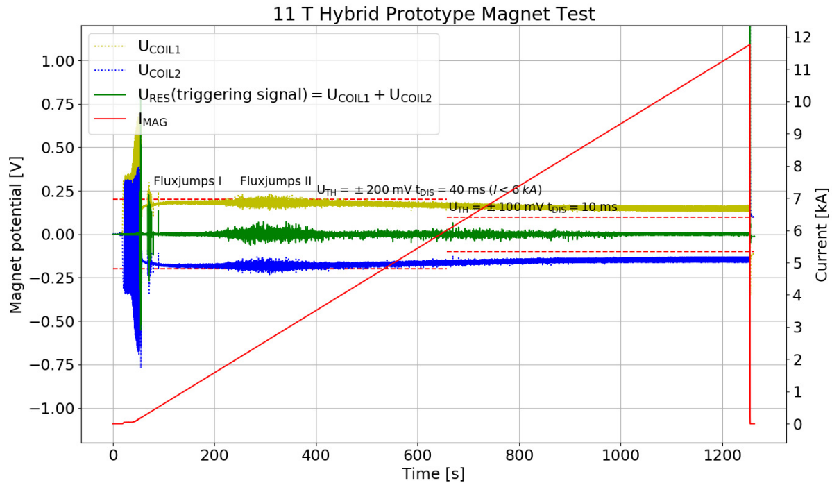
Figure 2: Recorded data of a training quench of a 11 T hybrid prototype magnet at I = 11762 A. The UQDS system has been configured with current depended detection settings to overcome the flux jump region at low currents. The system served as well as data acquisition system with 205.8 kS/s and an effective resolution of 687 \mu\text{V} at \pm 22.5 V input range. The quench detection settings are given by the threshold voltage U_{\text{TH}} and the evaluation and discrimination time t_{\text{DIS}} .
