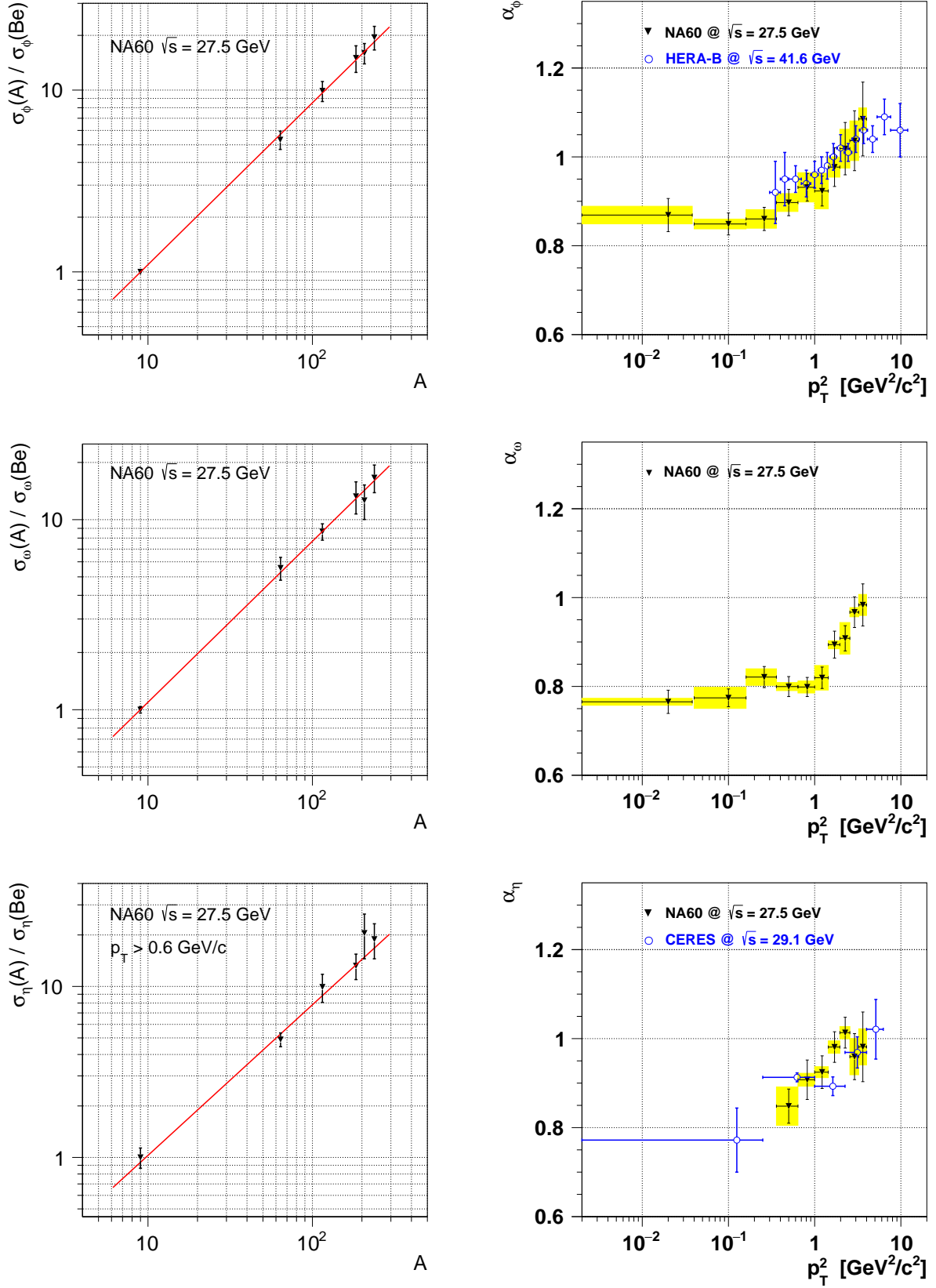
Fig. 5 Left column: fit on the relative production cross sections for the \omega , \phi and \eta mesons as a function of A, normalized to the Be or the Cu target. Right column: p_T dependence of the \alpha parameter for the \omega , \phi and \eta mesons.
