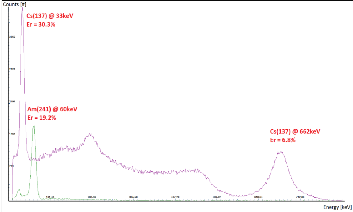
Figure 19. Spectra of ^{241}\text{Am} and ^{137}\text{Cs} source photons acquired with the SensL SiPM ArrayC-30035-16P and the EPIC [26] 15 \text{ } \emptyset \times 15 \text{ mm}^3 \text{LaBr}_3 crystal.
