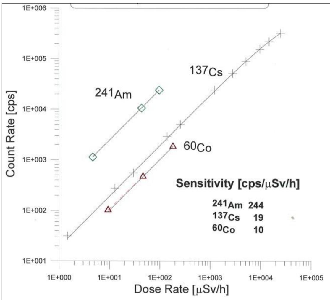
Figure 7. Cps to \mu\text{Sv/h} calibration factors for Unit 5.
