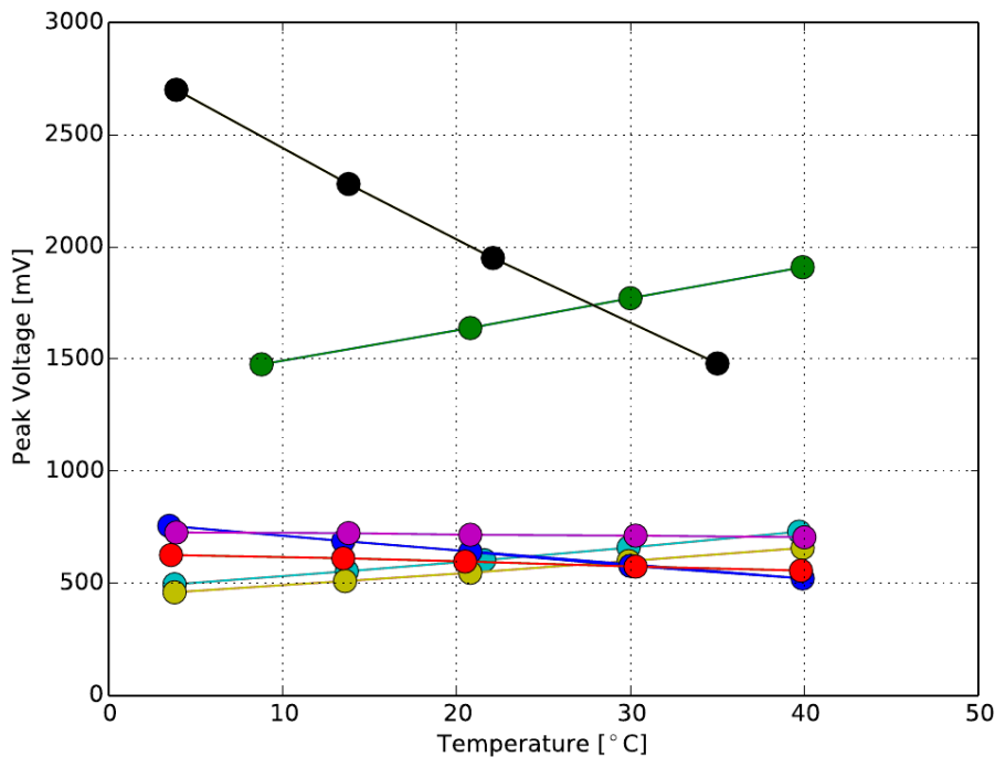
Figure 14. ^{137}\text{Cs} peak position as a function of temperature without (black curve, with slope -37.48\text{ mV} ) and with compensation for different values of R_{47} for Unit 5. The tested values for R_{47} are 75\text{ k}\Omega (green line, with slope 13.96\text{ mV} ), 78.6\text{ k}\Omega (light blue line, with slope 6.54\text{ mV} ), 80.6\text{ k}\Omega (yellow line, with slope 5.47\text{ mV} ), 105\text{ k}\Omega (violet line, with slope -0.606\text{ mV} ), 114\text{ k}\Omega (red line, with slope -1.975\text{ mV} ), 150\text{ k}\Omega (blue line, with slope -6.49\text{ mV} ).
