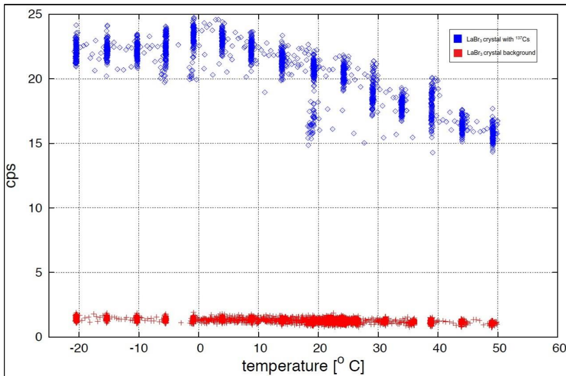
Figure 11. Count rate measurements with Unit 5 ( \text{LaBr}_3 ) as a function of temperature with a ^{137}\text{Cs} source (blue data) and without source (natural and \text{LaBr}_3 internal background, red data).
