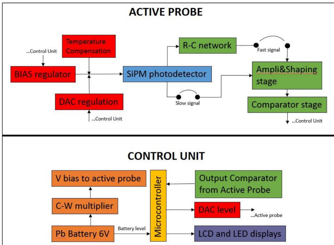
Figure 3. Block diagram of active probe and control unit. The Cockroft-Walton voltage multiplier and the red blocks in the active probe are shown in figure 4 and figure 5.
