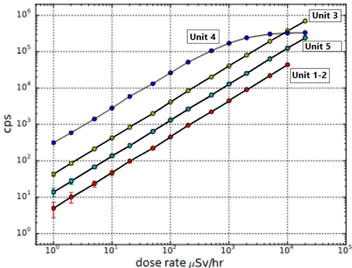
Figure 6. Count rate (counts per second, cps) versus dose rate linearity measurements on the five units. Units 1 and 2 equipped with a 4 \times 4 \times 15 \text{ mm}^3 LaBr 3 crystal overlap (red dots), Unit 5 (green dots) mounts the same crystal as Units 1 and 2 but has a lower energy threshold, Unit 3 (yellow dots) mounts a cylindrical 10 \emptyset \times 10 \text{ mm}^3 LaBr 3 crystal, Unit 4 (blue dots) mounts a cylindrical 25.4 \emptyset \times 25.4 \text{ mm}^3 NaI crystal.
