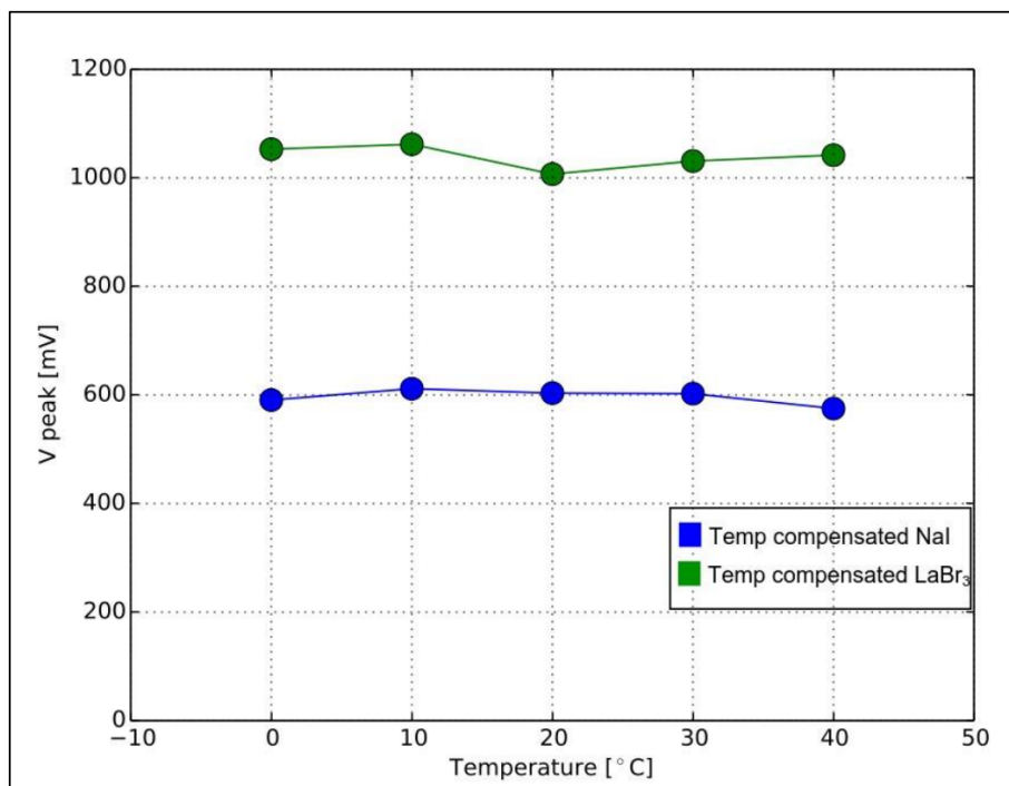
Figure 15. ^{137}\text{Cs} peak position as a function of temperature with compensation for R47 = 168 \text{ k}\Omega , comparing NaI (blue line) and LaBr 3 (green line) crystals in Unit 4.
