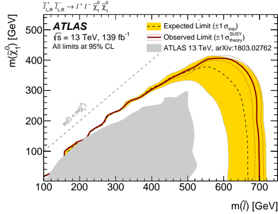
(c) \tilde{l}\tilde{l} production
