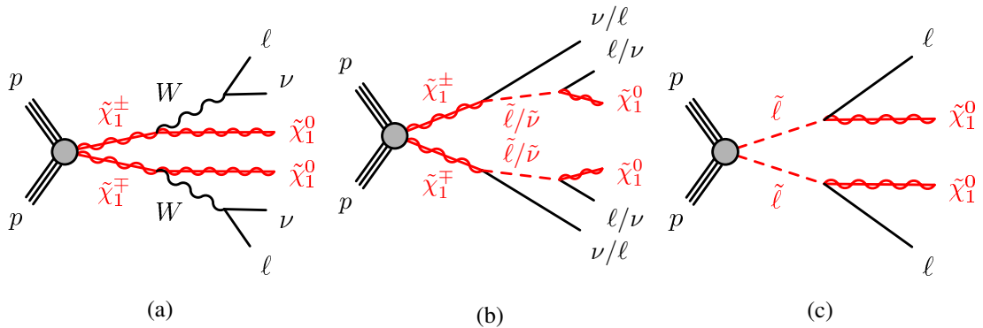
Figure 1: Diagrams of the supersymmetric models considered, with two leptons and weakly interacting particles in the final state: (a) \tilde{\chi}_1^+ \tilde{\chi}_1^- production with W-boson-mediated decays, (b) \tilde{\chi}_1^+ \tilde{\chi}_1^- production with slepton/sneutrino-mediated decays and (c) slepton pair production. In the model with intermediate sleptons, all three flavours ( \tilde{e} , \tilde{\mu} , \tilde{\tau} ) are included, while only \tilde{e} and \tilde{\mu} are included in the direct slepton model. In the final state, \ell stands for an electron or muon, which can be produced directly or, in the case of (a) and (b) only, via a leptonically decaying \tau -lepton with additional neutrinos.
