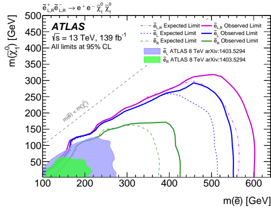
(a) \tilde{e}\tilde{e} production
