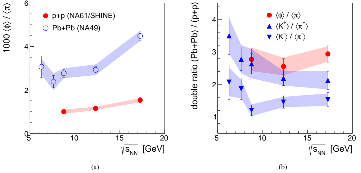
Figure 15: Energy dependence of (a) ratios of total yields of \phi mesons to mean total yields for pions (Eq. (12)) in p + p and Pb + Pb, (b) double ratios (see text). Full red circles correspond to results of this analysis, Pb + Pb data come from NA49 [18, 41, 42], while p + p kaon and pion data are taken from Ref. [43]. Possible correlations of uncertainties of yields within the same reaction are neglected. This may lead to a slight overestimation of the indicated uncertainties.
