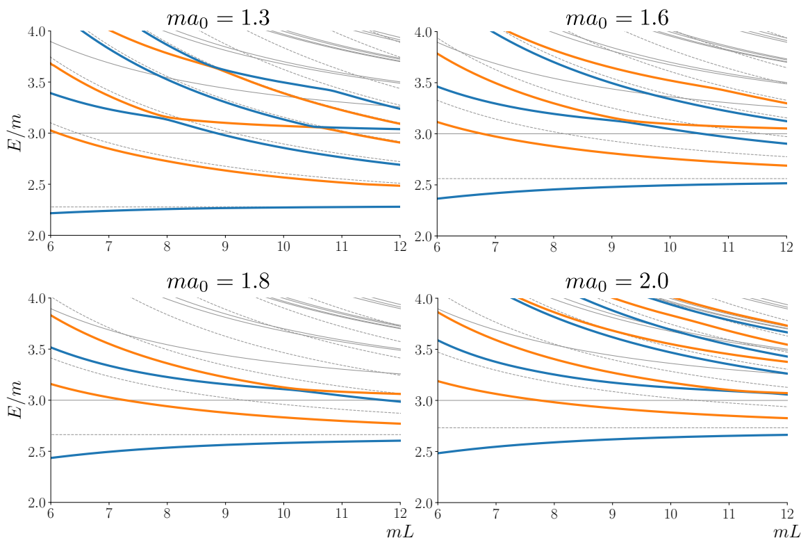
Figure 4. The spectrum for four values of ma_0 and \mathcal{K}_{\text{df},3}^{\text{iso}} = 0 as a function of mL . All four values lead to relativistic two-particle bound states. Solid grey lines show the energies of three noninteracting particles (1+1+1 states), while dashed grey lines give the energies of noninteracting dimer + particle states (2+1 states). The interacting energy levels are shown in alternating colors to emphasize the avoided level crossings. Although it is not apparent from these plots, by going to larger values of mL we find that the lowest state for ma_0 = 1.6, 1.8, and 2.0 is a trimer, while that for ma_0 = 1.3 asymptotes to the dimer + particle energy as mL \rightarrow \infty . See the text for further discussion.
