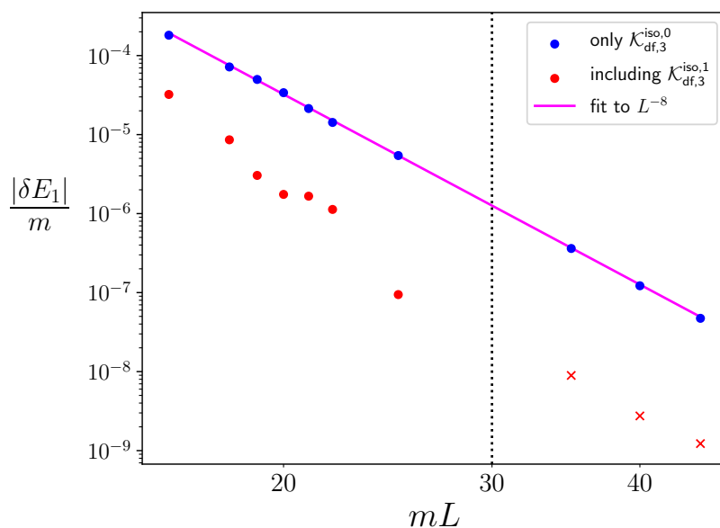
Figure 16. |\delta E_1| as a function of mL when tuning with only a constant \mathcal{K}_{\text{df},3}^{\text{iso}} (filled blue circles) or with the linear dependence on \Delta given in eq. (A.6) (filled red circles and crosses). The solid (magenta) line shows a fit to the blue points assuming an L^{-8} -dependence. The vertical line indicates the value of mL at which the tuning is done. Thus the corresponding red point vanishes at this value and is not shown. \delta E_1 is positive for the red circles and negative for the red crosses.
