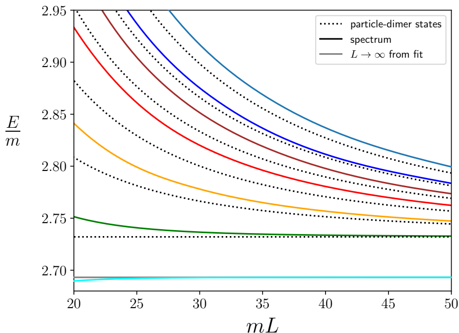
Figure 5. Low-lying spectrum for ma_0 = 2 and \mathcal{K}_{\text{df},3}^{\text{iso}} = 0 for larger mL . This is the continuation to larger volumes of the spectrum shown in the bottom right-hand panel of figure 4. Note the highly compressed vertical scale. The horizontal line for the lowest level gives the L \rightarrow \infty asymptote for the trimer energy, using a fit described in the text.
