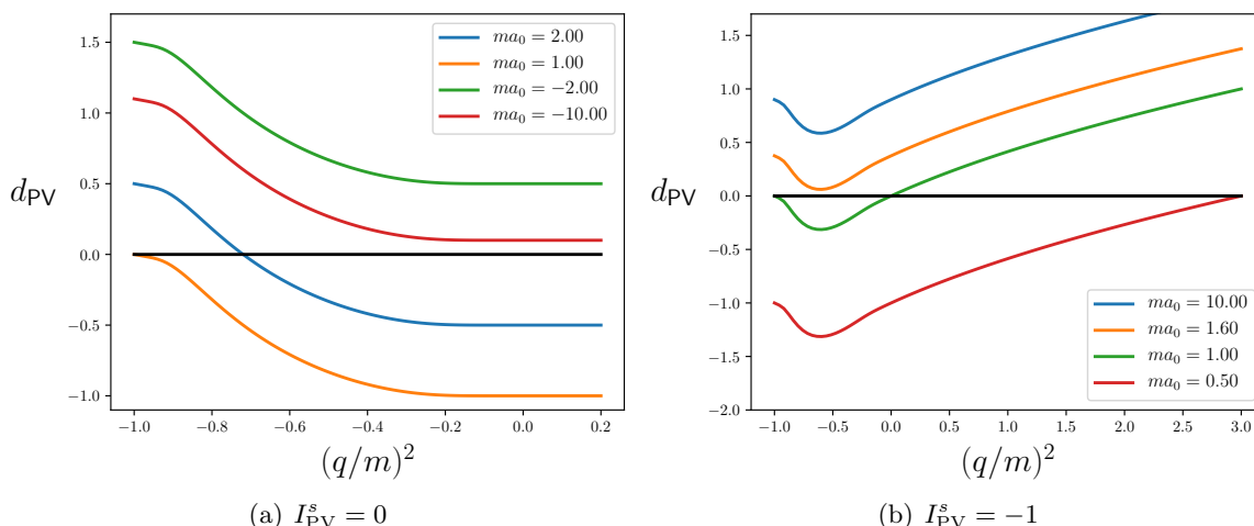
Figure 2. Plots of the denominator of \tilde{\mathcal{K}}_2^s , d_{PV}(q^2) , vs. q^2/m^2 for a range of choices of am with I_{PV}^s = 0 (left) and I_{PV}^s = -1 (right). There is a pole in \tilde{\mathcal{K}}_2^s whenever d_{PV}(q^2) vanishes. See text for further discussion.
