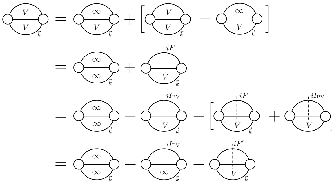
Figure 1. Illustration of the previous and modified PV prescriptions used in the analysis of the three-particle correlation function, for the simplest diagram. Loops containing the symbol “ \infty ” are integrated, while those containing a “ V ” have the spatial components of the momentum summed. All integrals use the PV prescription. In the first line the upper sum is replaced by an integral plus a sum-integral difference. The latter can be replaced by an F cut, as shown in the second line, while the lower loop sum can be replaced by an integral in the first term on this line. In the third line we subtract and add the I_{\text{PV}}^s cut. The final line shows that this new cut can be absorbed into the modified F , leaving a modified PV prescription for the upper loop integral.
