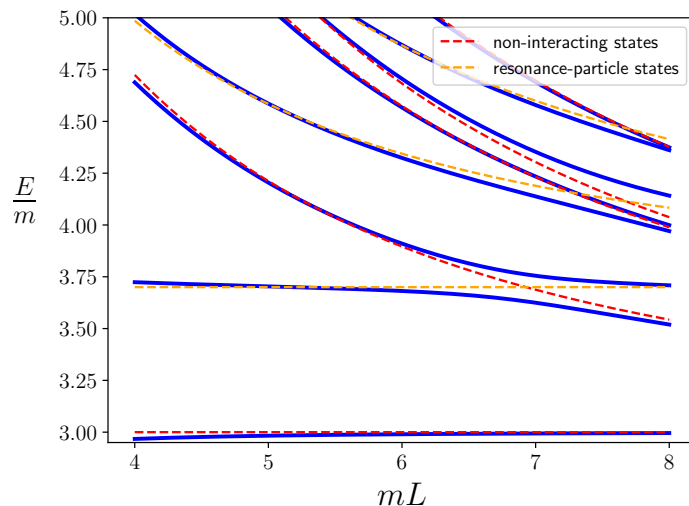
Figure 11. Three-particle spectrum (solid blue lines) in the isotropic approximation in the presence of a two-particle resonance with g = 1 , m_R = 2.7m and \mathcal{K}_{df,3} = 0 . Noninteracting three-particle states (red dashed lines) and noninteracting particle + resonance states (orange dashed lines) are shown for comparison.
