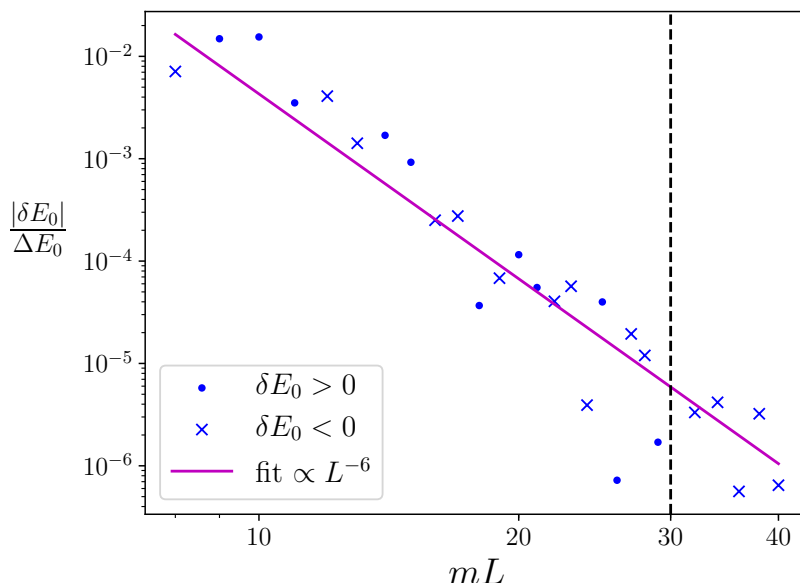
Figure 14. I_{\text{PV}} -dependence of the ground-state energy E_0(L) , with \delta E_0 defined in eq. (A.3). We plot the ratio to \Delta E_0 = E_0 - 3m in order to give a sense of the relative size of the shift. The vertical line at mL = 30 indicates the point at which matching is performed, so that \delta E_0 vanishes.
