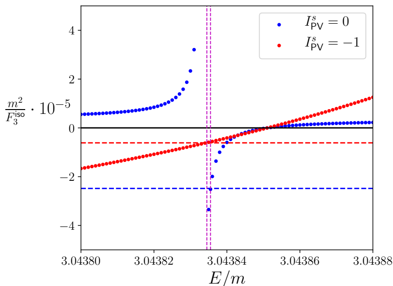
Figure 15. As for figure 13 but for the first excited state. The dashed magenta lines correspond to the values of E_1(I_{\text{PV}} = 0; mL = 30) and E_1(I_{\text{PV}} = -1; mL = 30) obtained from the constant approximations m^2\mathcal{K}_{\text{df},3}^{\text{iso}}(I_{\text{PV}} = 0) = 2.4828 \cdot 10^5 and m^2\mathcal{K}_{\text{df},3}^{\text{iso}}(I_{\text{PV}} = -1) = 6.1365 \cdot 10^4 . The discrepancy between the two magenta lines is due to our neglect of the higher-order terms in the threshold expansion of \mathcal{K}_{\text{df},3} .
