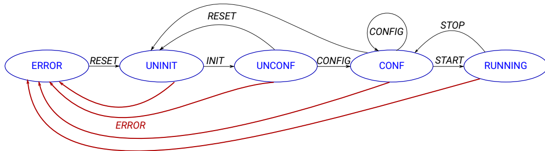
Figure 2. Finite State Machine of EUDAQ2. States are displayed in blue, commands in black and error handling in red. For the successful initialization and configuration of EUDAQ2, valid initialization and configuration files need to be provided.
