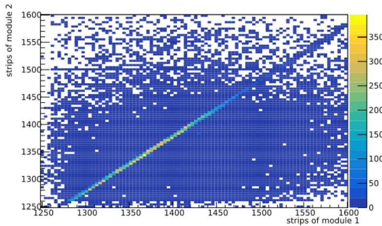
Figure 5. Spatial correlations of two LYCORIS strip sensor modules from example data taken with the EUDAQ2 KPiX user module at DESY II Test Beam Facility.
