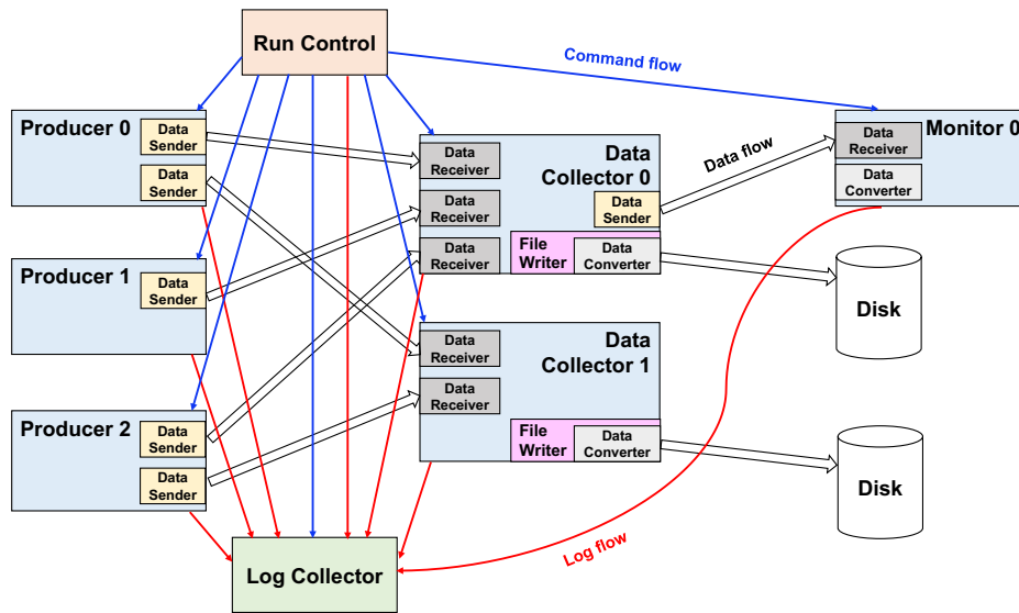
Figure 1. A schematic view of the EUDAQ2 architecture.
