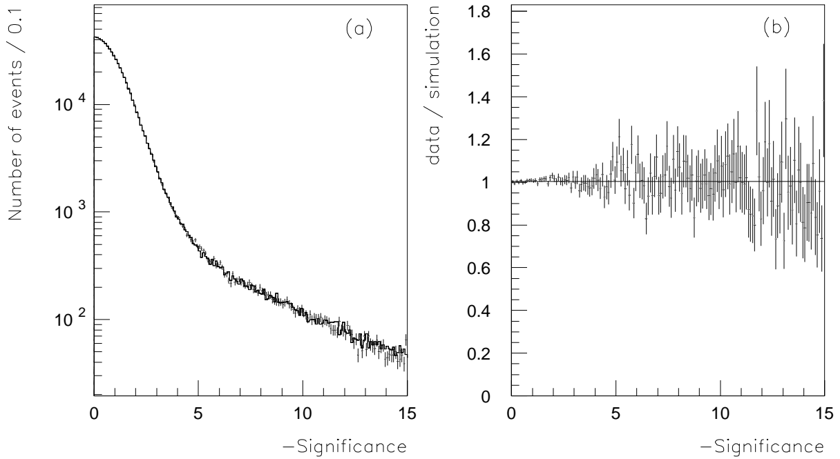
Figure 3: (a): Negative significance distribution for data (points with errors) and for simulation (histogram). (b) The ratio of negative significance distributions of data and simulation for tracks with negative impact parameters.
