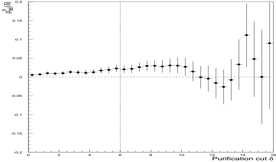
Figure 13: Double tag hemisphere correlation factor ( I = 6, J = 6 ), as a function of \delta . For the standard cut at \delta = 6 , the value of \rho_{66}^b is 0.018 \pm 0.010 and it remains rather stable over the whole range. Note that, by definition of \rho_{66}^b , the points are bin-to-bin correlated.
