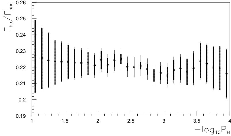
Figure 5: The value of \Gamma_{b\bar{b}}/\Gamma_{had} as a function of the cut on -\log_{10} P_H . Both the total errors (narrow bars) and uncorrelated ones relative to the cut -\log_{10} P_H > 2.5 (wider bars) are shown.
