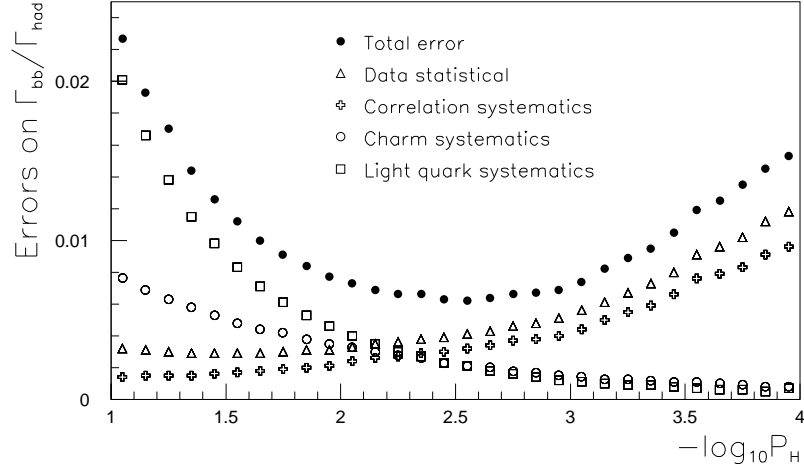
Figure 4: Errors of the measurement of \Gamma_{b\bar{b}}/\Gamma_{had} as a function of the cut on -\log_{10} P_H .
