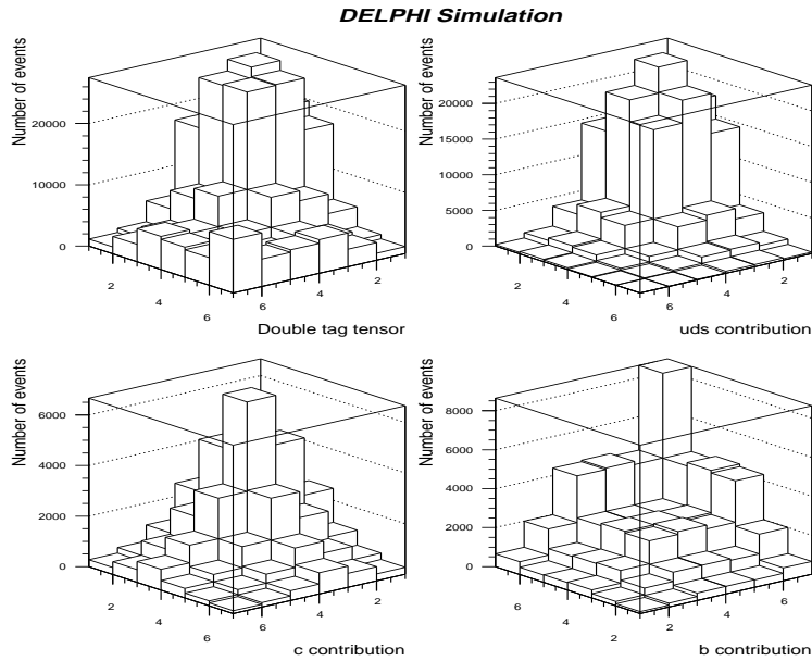
Figure 9: Population of the double tag tensor with their uds , c and b contributions for simulated events. Note that the axes for the b contribution are rotated by 180 degrees with respect to the other plots.
