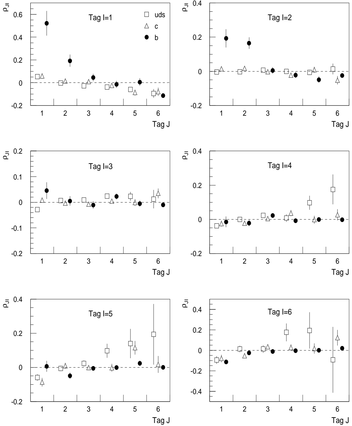
Figure 12: Double tag hemisphere correlation factors \rho_{JI}^l for simulation.
