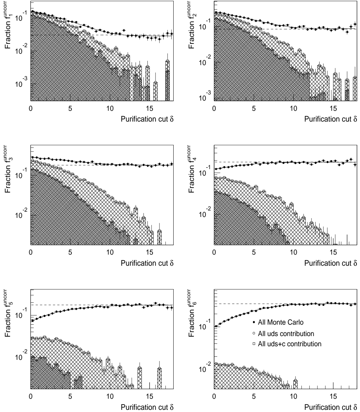
Figure 10: f_I^{uncorr}(\delta) distributions with their asymptotic fits (see text) for simulation. If hemispheres are independent, f_I^{uncorr}(\delta) should tend asymptotically to C_I^b when \delta increases. The big cross-hatched area indicates the c contamination while the small cross-hatched area is the uds contribution. No asymptotical irreducible uds and c background is observed in the asymptotic region, particularly in f_4 , f_5 and f_6 distributions which are the most significant for the extraction of R_b . The dashed horizontal lines show the true values for C_I^b .
