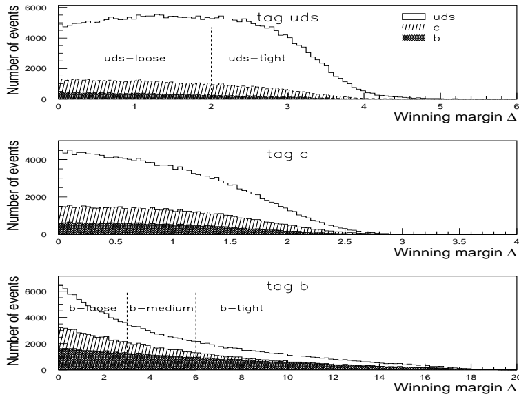
Figure 7: Distributions obtained from the simulation of the winning margin \Delta in the uds , c and b hemisphere tag. The filled areas show the different heavy flavour contributions to the events in a given tag. The dashed lines show the cuts to separate the 6 different categories.
