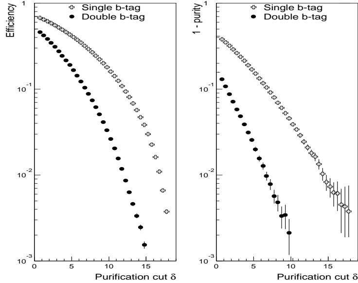
Figure 8: Efficiency and purity of the single and double hemisphere b tags versus the value of the clear winning cut \delta = \Delta_b^{cut} for simulated events. The purity is plotted in the form 1 - \text{purity} .
