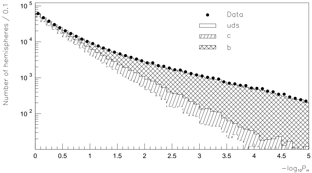
Figure 2: Distribution of -\log_{10}(P_H) for data and different flavour contributions from the simulation.
