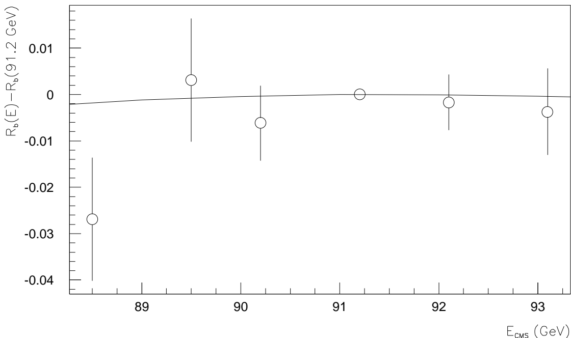
Figure 6: The difference \Gamma_{b\bar{b}} / \Gamma_{had}(E_{CMS}) - \Gamma_{b\bar{b}} / \Gamma_{had}(E_{CMS} = 91.2 \text{ GeV}) . The Standard Model prediction is shown by the curve.
