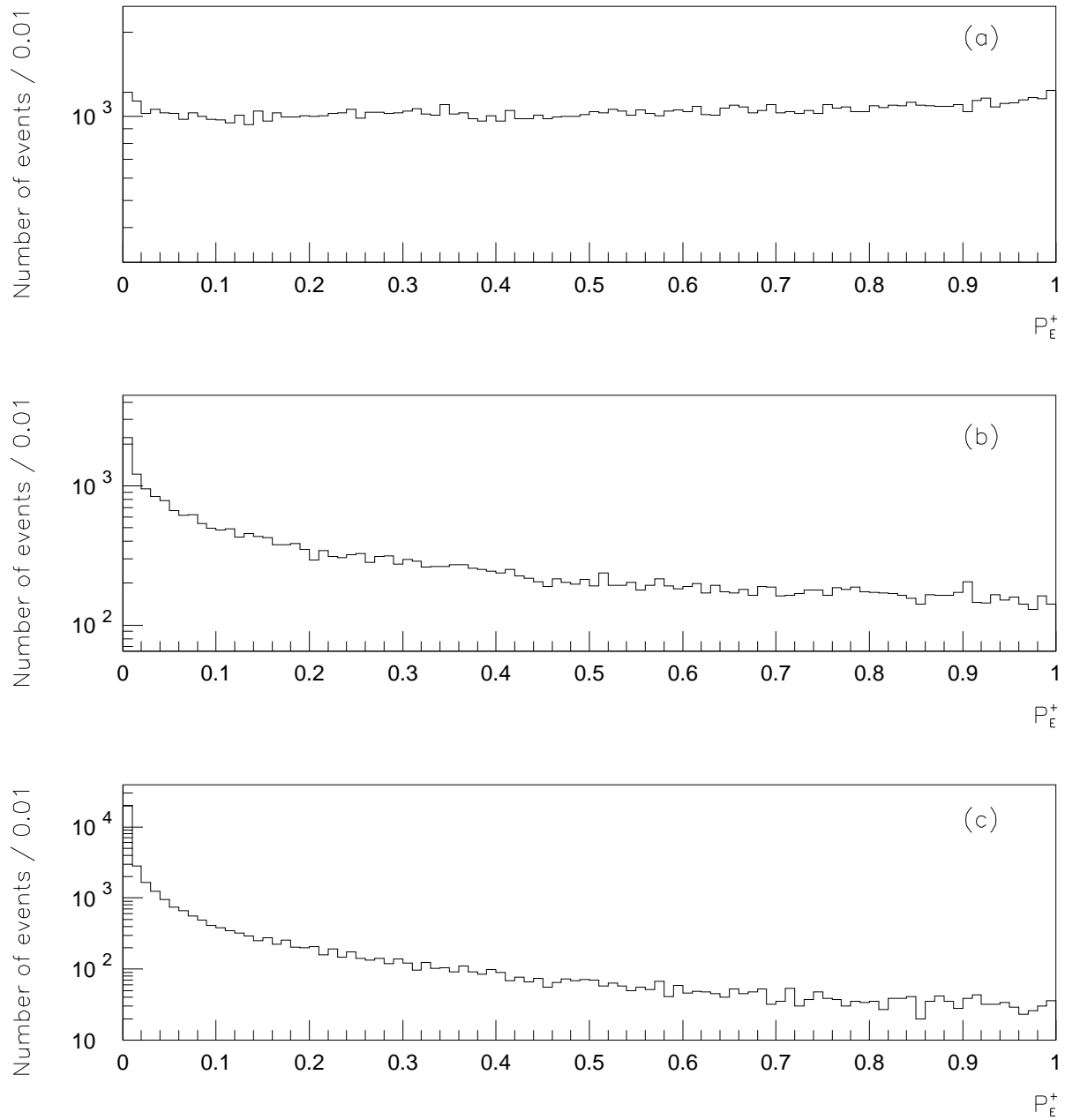
Figure 1: Distribution of event simulated probability P_E^+ for particles with positive impact parameters, for light quark events (a), charm quark events (b) and b -quark events(c).
