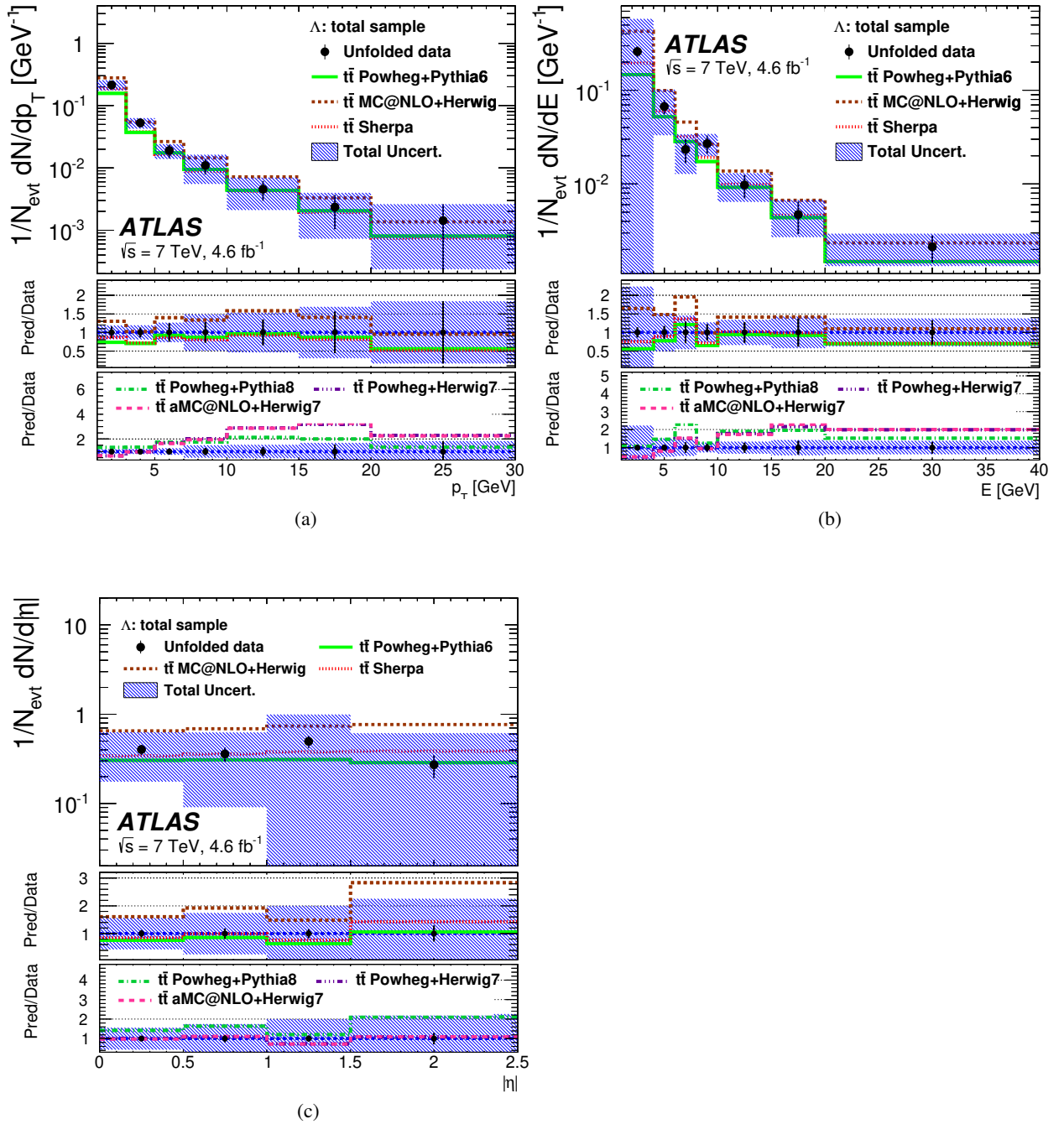
Figure 11: Kinematic characteristics for the total \Lambda production, for corrected data and particle-level MC events simulated with the POWHEG+PYTHIA6, MC@NLO+HERWIG, SHERPA, POWHEG+PYTHIA8, POWHEG+HERWIG7 and aMC@NLO+HERWIG7 generators. Total uncertainties are represented by the shaded area. Statistical uncertainties for MC samples are negligible in comparison with data.
