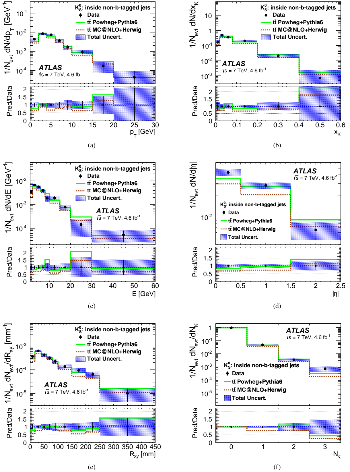
Figure 4: Kinematic characteristics for K_S^0 production inside non- b -tagged jets, for data and detector-level MC events simulated with the POWHEG+PYTHIA6 and MC@NLO+HERWIG generators. Total uncertainties are represented by the shaded area. Statistical uncertainties for MC samples are negligible in comparison with data.
