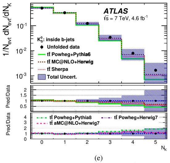
Figure 8: Kinematic characteristics for K_S^0 production inside b -jets, for corrected data and particle-level MC events simulated with the POWHEG+PYTHIA6, MC@NLO+HERWIG, SHERPA, POWHEG+PYTHIA8, POWHEG+HERWIG7 and aMC@NLO+HERWIG7 generators. Total uncertainties are represented by the shaded area. Statistical uncertainties for MC samples are negligible in comparison with data.
