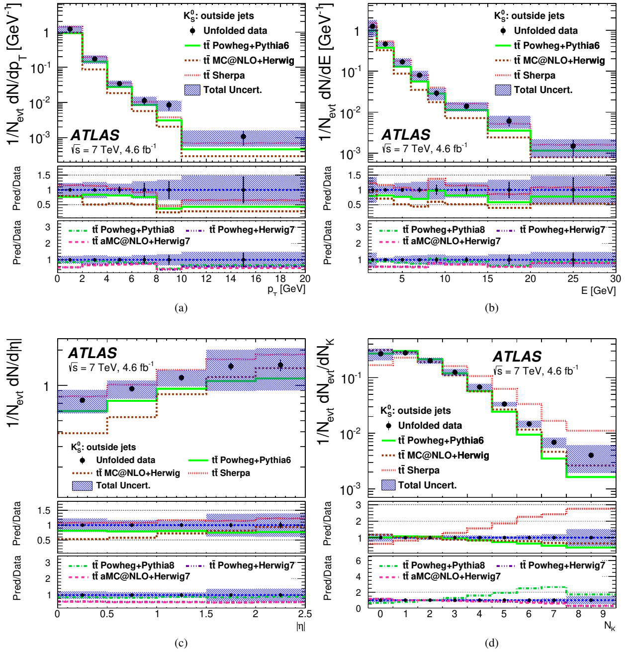
Figure 10: Kinematic characteristics for K_S^0 production not associated with jets, for corrected data and particle-level MC events simulated with the POWHEG+PYTHIA6, MC@NLO+HERWIG, SHERPA, POWHEG+PYTHIA8, POWHEG+HERWIG7 and aMC@NLO+HERWIG7 generators. Total uncertainties are represented by the shaded area. Statistical uncertainties for MC samples are negligible in comparison with data.
