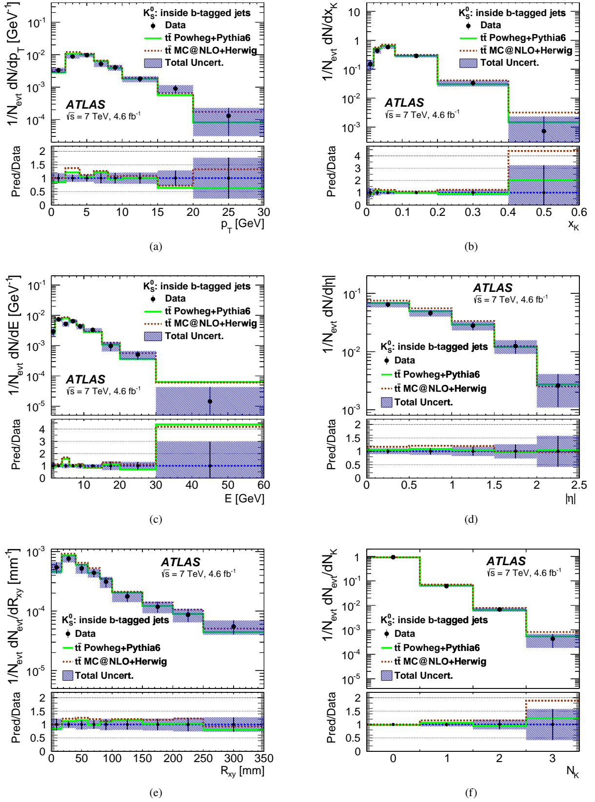
Figure 3: Kinematic characteristics for K_S^0 production inside b -tagged jets, for data and detector-level MC events simulated with the POWHEG+PYTHIA6 and MC@NLO+HERWIG generators. Total uncertainties are represented by the shaded area. Statistical uncertainties for MC samples are negligible in comparison with data.
