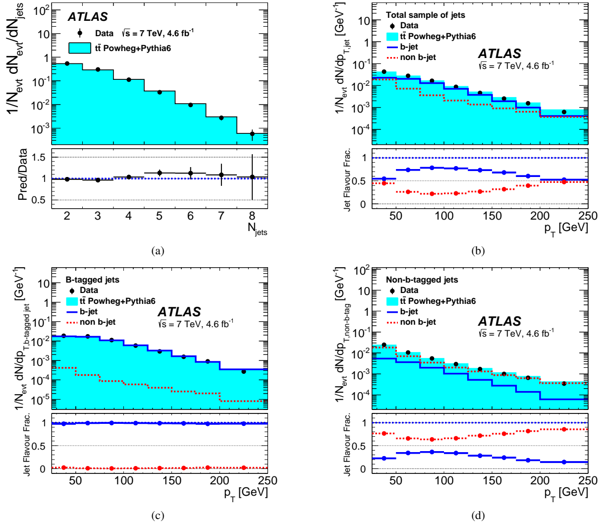
Figure 1: Spectra of (a) jet multiplicity N_{\text{jets}} and (b) jet p_{\text{T}} in data compared with t\bar{t} POWHEG+PYTHIA6 predictions at detector level. The expected b -jet flavour fractions for (c) b -tagged and (d) non- b -tagged jets as a function of jet p_{\text{T}} are also compared with data. These distributions are normalised to the total number of selected events in data or MC predictions.
