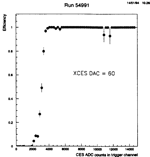
Fig. 1. The turn-on efficiency for XCES bits as a function of the CES energy deposition in a 4-wire strip, expressed here in ADC counts. 1 \text{ GeV} \approx 800 counts. The DAC threshold that determines the turn-on point is adjustable and is shown here at its nominal value.
