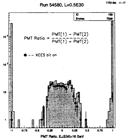
Fig. 2. The phototube ratio R , defined as the difference between the two phototube energies in a tower divided by their sum. Single-phototube spikes show up at \pm 1 , and dominate the physics rate in this low-luminosity run. The points show R for towers with an OR-bit turned on.
