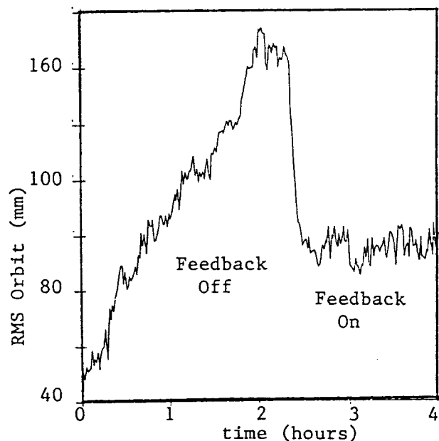
Figure 4. Example of SVD orbit control on SPEAR.
