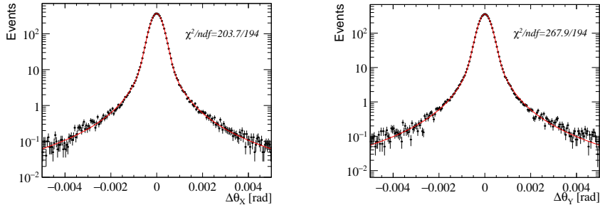
Figure 14. x -projection (Left) and y -projection (Right) of the scattering angle from 12 GeV e^- from MC GEANT4 simulation with 8 mm target compared with the results of the fit. Details are given in the text.
