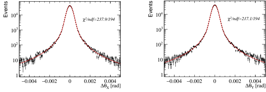
Figure 11. x -projection (Left) and y -projection (Right) of the scattering angle from 12 GeV e^- for data with 8 mm target compared with the results of the fit. Details are given in the text.
