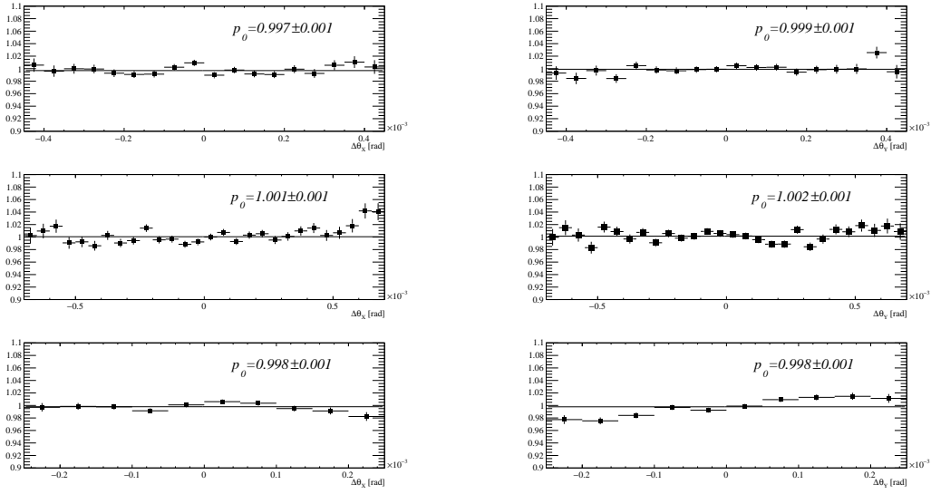
Figure 8. Data/MC ratio of x -projection (Left) and y -projection (Right) of the scattering angle between data and GEANT4 in the core region (90% events): (upper) 12 GeV e^- with 20 mm C target; (center) 12 GeV e^- with 8 mm C target; (lower) 20 GeV e^- with 8 mm C target.
