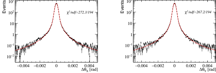
Figure 16. x -projection (Left) and y -projection (Right) of the scattering angle from 20 GeV e^- from MC GEANT4 simulation with 8 mm target compared with the results of the fit. Details are given in the text.
