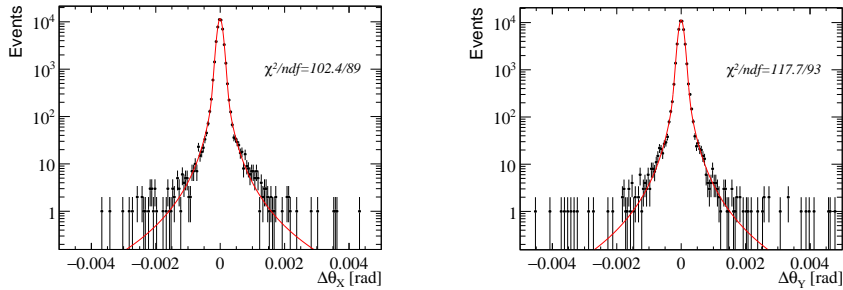
Figure 10. x -projection (Left) and y -projection (Right) of the scattering angle from 20 GeV alignment e^- data ( i.e. without target) compared with the results of the fit.
