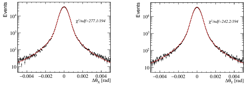
Figure 12. x -projection (Left) and y -projection (Right) of the scattering angle from 12 GeV e^- for data with 20 mm target compared with the results of the fit. Details are given in the text.
