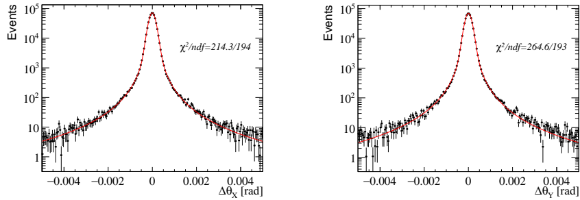
Figure 13. x -projection (Left) and y -projection (Right) of the scattering angle from 20 GeV e^- for data with 8 mm target compared with the results of the fit. Details are given in the text.
