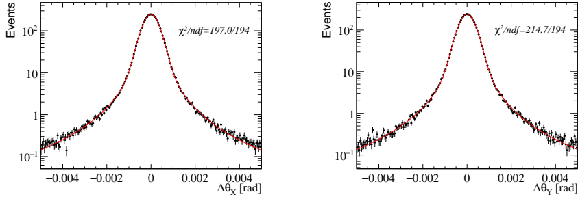
Figure 15. x -projection (Left) and y -projection (Right) of the scattering angle from 12 GeV e^- from MC GEANT4 simulation with 20 mm target compared with the results of the fit. Details are given in the text.
