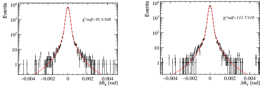
Figure 9. x -projection (Left) and y -projection (Right) of the scattering angle from 12 GeV e^- alignment data ( i.e. without target) compared with the results of the fit.
