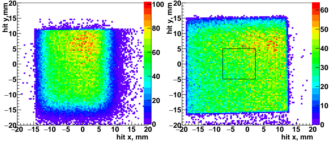
Figure 3. Hit occupancy of the electron beam of 12 GeV in the upstream region, (Left) first plane; (Right) second plane.
