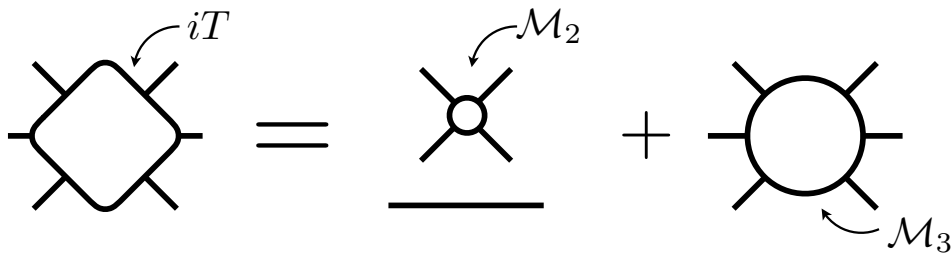
FIG. 1: The two types of contribution to the three-particle T matrix. \mathcal{M}_3 is the fully-connected amplitude.
