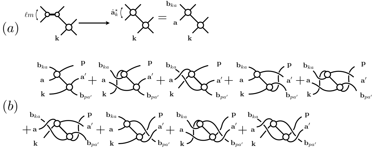
FIG. 2: Schematic representation of the definition of symmetrization given in Eq. (18), using the example of the leading term in \mathcal{D}^{(u,u)} . (a) Basis transformation from the k, \ell, m to the one in terms of three momenta; (b) Summing over permutations of assignments of external momenta. Open circles represent \mathcal{M}_2 , which is itself symmetric under particle interchange. The third momentum on the left-hand side is given by \mathbf{b}_{ka} = \mathbf{P} - \mathbf{k} - \mathbf{a} , with \mathbf{b}_{pa'} defined similarly. See main text for further explanation.
