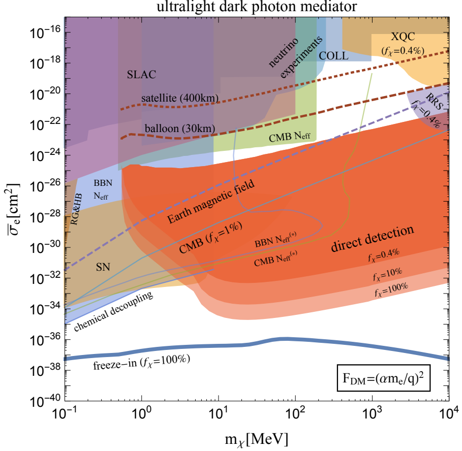
Figure 11: Discovery reach (thick red dashed lines) for a silicon dark matter detector with single-electron sensitivity on a balloon (satellite) assuming an exposure of 1 gram-hour ( 0.1 gram-month) and 10^6 ( 10^9 ) background events, together with constraints on dark matter interacting with a massive, ultralight dark photon. Also shown are cooling constraints from supernovae 1987A (brown, “SN”) [76], as well as Red-Giant and Horizontal-Branch stars (brown, “RG&HB”) [71]; constraints from measurements of the number of relativistic degrees of freedom from the CMB (light green, “CMB N_{\text{eff}} ”) and BBN (blue, “BBN N_{\text{eff}} ”) [73, 108], and from searches for milli-charged particles at SLAC (purple, “SLAC”) [77], colliders (blue, “COLL”) [71, 112], and at LSND and MiniBooNE (green, “neutrino experiments”) [78]; and the direct-detection constraints derived in this paper from SENSEI, CDMS-HV, XENON10, XENON100, and DarkSide-50 (combined into one red-shaded region, labelled “direct detection”), as well as from RRS (purple) and XQC (light orange) [54]. We also show for comparison the “freeze-in” line along which DM obtains the correct relic density in this model [4, 113]. The region at high cross sections is unconstrained from CMB measurements if this DM particle only makes up a subdominant component ( f_\chi \lesssim 0.4\% ) of the total observed DM abundance [70]; for comparison, we show the CMB constraint for a fractional abundance of f_\chi = 1\% (blue line, “CMB ( f_\chi = 1\% )”), in which case the entire region at high cross section is disfavored [114]. For the N_{\text{eff}} constraints from the CMB and BBN, we assume that the dark gauge coupling is sufficiently small to avoid the production of dark photons at early times; for large values of the dark gauge coupling, the bounds would be given by the thin blue and green lines (“BBN N_{\text{eff}}^{(*)} ”) and “CMB N_{\text{eff}}^{(*)} ”) [71].
