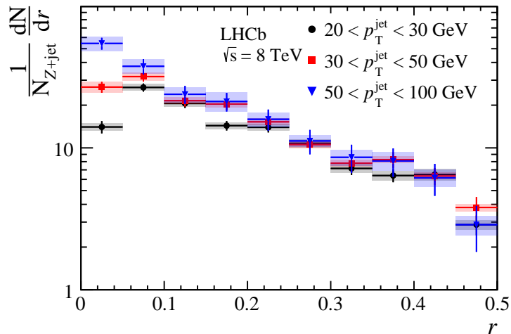
Figure 3: Radial profile distributions of hadrons with respect to the jet axis in three bins of jet p_T . The bars (boxes) show the statistical (systematic) uncertainties.
