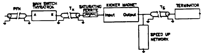
Figure 1: Block diagram of kicker magnet system
