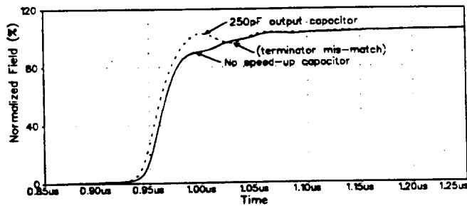
Figure 2: Measured field, normalized, with and without an output speed-up capacitor
