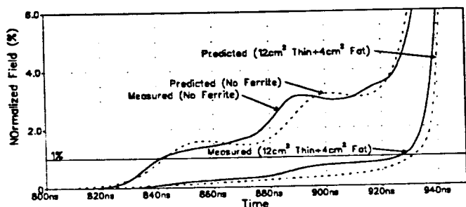
Figure 4: Measured and predicted pre-pulse field, with and without ferrite
