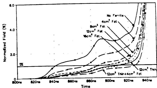
Figure 3: Measured normalized pre-pulse field for various geometries of saturating ferrite
