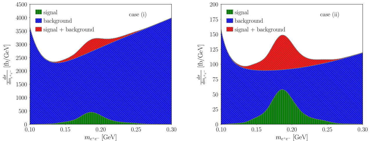
FIG. 4: The differential cross sections with respect to the e^+e^- invariant mass for the expected \mathcal{TM} signal and combinatorial background at LHCb, assuming the normalization in Tab. I for case (i) and (ii). Global efficiencies of 20% and 6% are assumed to reconstruct the \mathcal{TM} and \mathcal{TM} plus photon candidates, respectively. In these conditions, a 5\sigma observation would be possible with an integrated luminosity of 15\text{fb}^{-1} in case (i) and of 30\text{fb}^{-1} in case (ii). The invariant mass resolution of the signal is described in the text. The shift observed in the central position of the signal peak, due to the lack of reconstructed bremsstrahlung from the electrons, is compatible with that of Ref. [44]. For the combinatorial background, the resulting invariant mass distribution is obtained from simulation.
