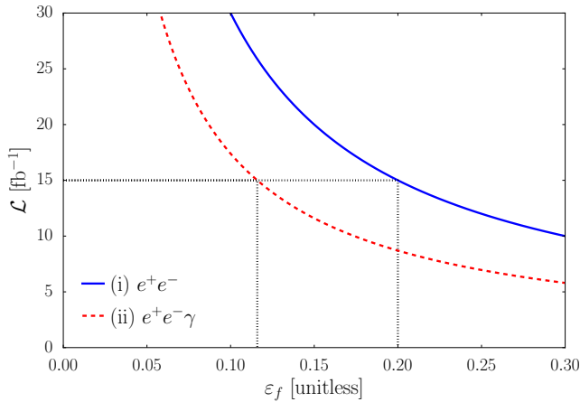
FIG. 3: The required integrated luminosity for a 5\sigma_{\text{stat}} discovery of \mathcal{T}\mathcal{M} as function of the final reconstruction efficiency, \varepsilon_f for the proposed (blue) e^+e^- and (red) e^+e^-\gamma searches.
