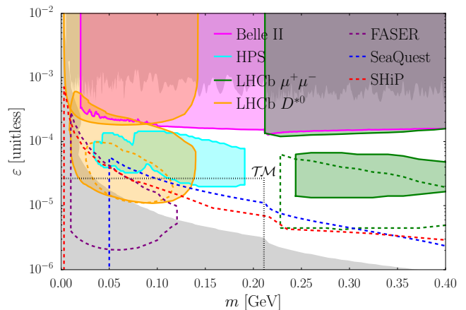
FIG. 1: Dark photon parameter space in dark photon mass and kinetic mixing with (gray) previous limits and future reach from (magenta) Belle II, (purple) FASER, (cyan) HPS, and (green/yellow) LHCb. \mathcal{TM} corresponds to the marked point, using Eqs. (2) and (3).
