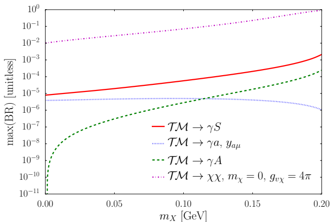
FIG. 5: \mathcal{T}\mathcal{M} branching ratio to BSM final states in Eqs. (C5)–(C8) which are allowed by (g-2)_\mu at the 5\sigma .
