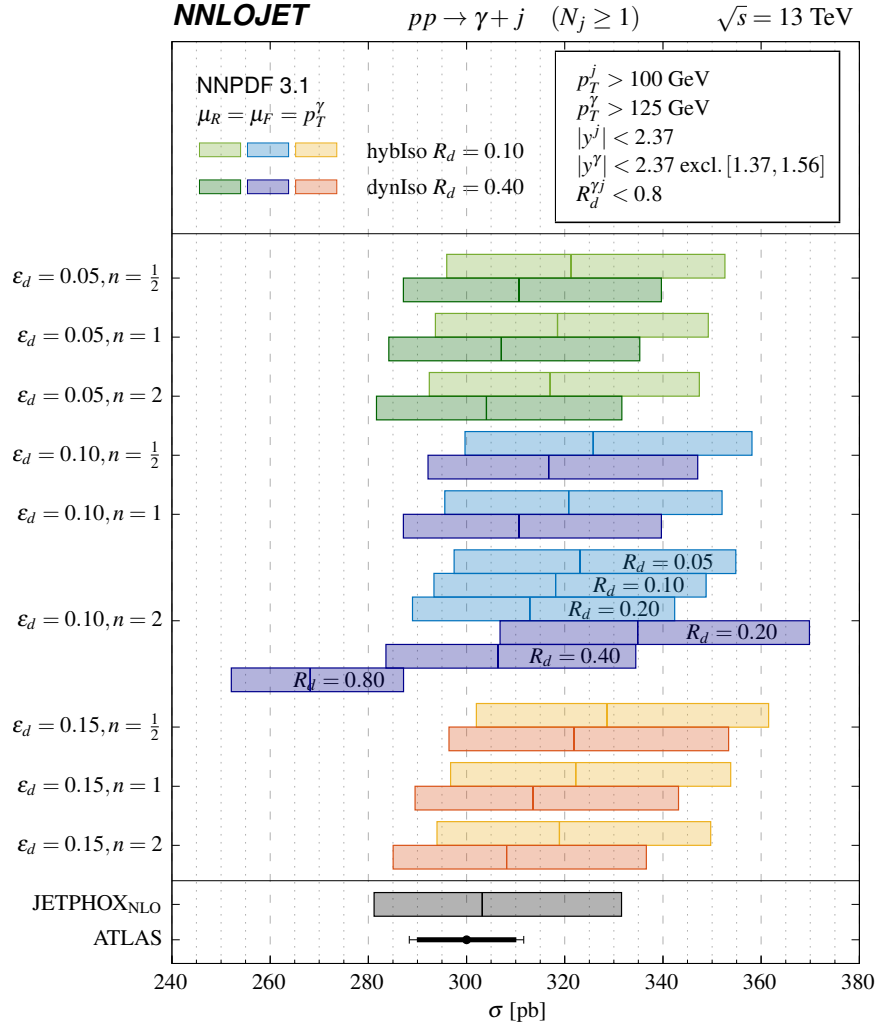
Figure 1. Total cross section for different parameter choices ( \varepsilon_d = 0.05, 0.1, 0.15 , n = \frac{1}{2}, 1, 2 ) for both dynamical photon isolation ( dynIso ) [30] (dark colours) and the dynamical cone part of the hybrid photon isolation ( hybIso ) (light colours). The default cone size for dynIso is R_d = 0.4 , while for hybIso it is R_d = 0.1 . For the specific parameter choice \varepsilon_d = 0.1, n = 2 we also investigate variations of the cone size by factors \frac{1}{2} and 2. The fixed cone parameters of the hybrid isolation are chosen according to the ATLAS measurement [17]. The fixIso prediction (using JETPHOX [36]) and the ATLAS measurement are shown for comparison.
