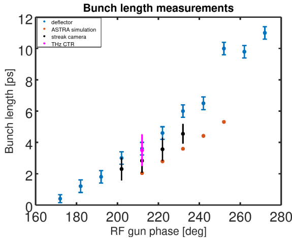
Figure 4: Bunch length experimental measurements with RF deflector, simulations, streak camera and THz radiation.
