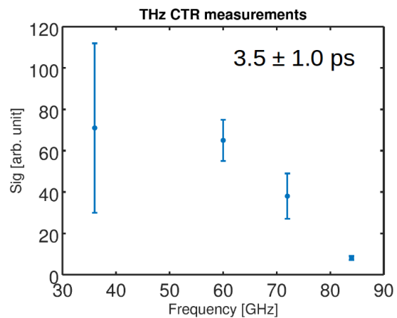
Figure 6: Bunch length experimental measurements from coherent transition radiation (CTR) recorded by zero-biased Schottky diodes.
