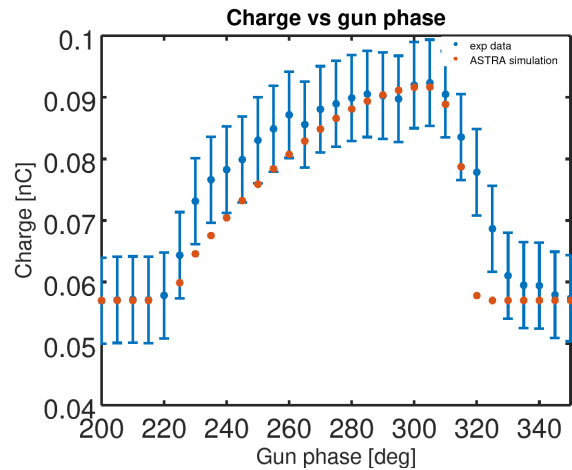
Figure 2: Comparison between the experimental extracted charge at ICT vs gun phase (blue line) and ASTRA simulation (orange line).
