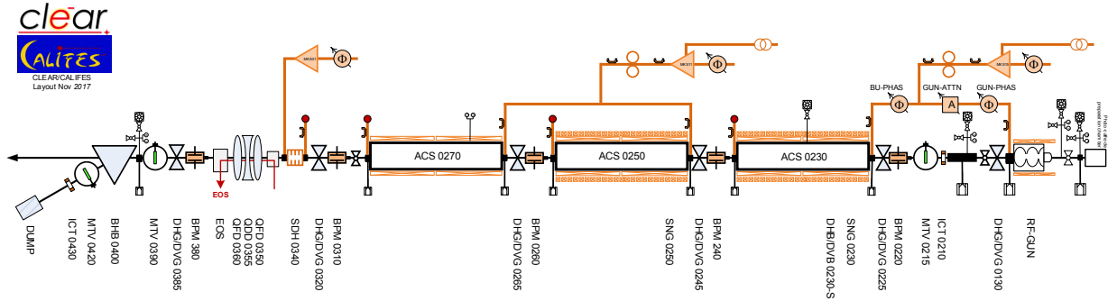
Figure 1: CLEAR accelerator layout.
