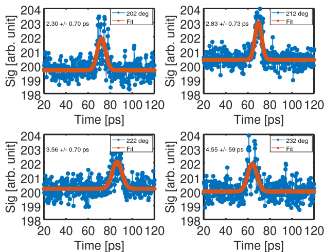
Figure 5: Bunch experimental temporal profiles recorded by the streak camera, for different RF gun phases.
