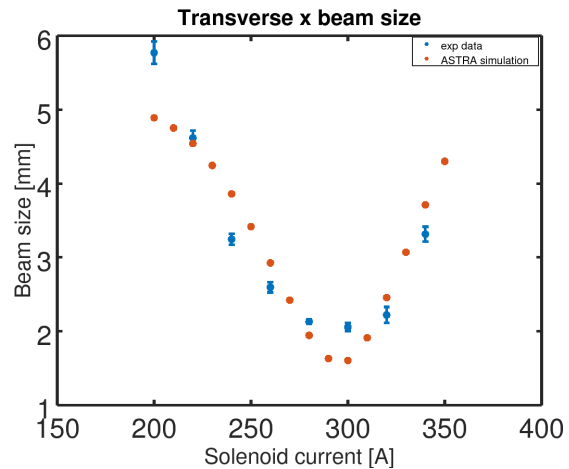
Figure 3: Comparison between the transverse beam size at ICT vs focusing solenoid current (blue line) and ASTRA simulation (orange line).
