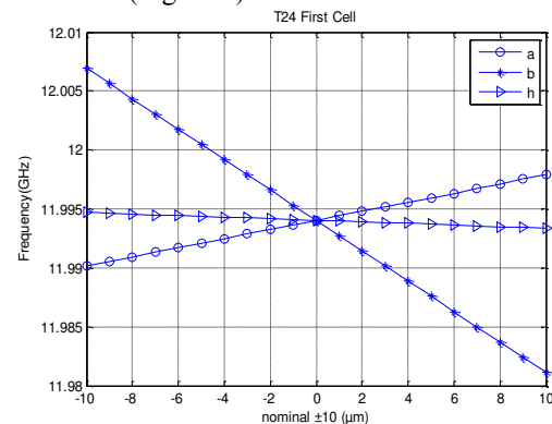
Figure 3: Frequency sensitivity of T24 cell.
