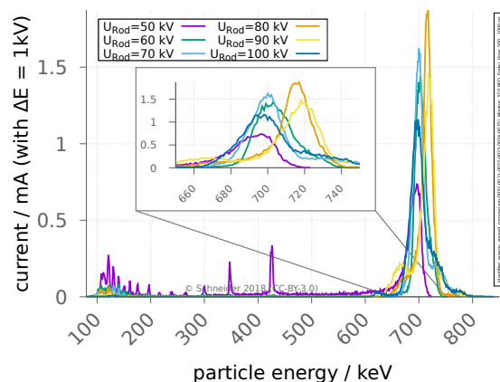
Figure 6: Energy histogram of a 120 keV, 50 mA proton beam downstream the RFQ in acceleration mode at rod voltages of U_{\text{Rod}} = 50 kV...100 kV.
