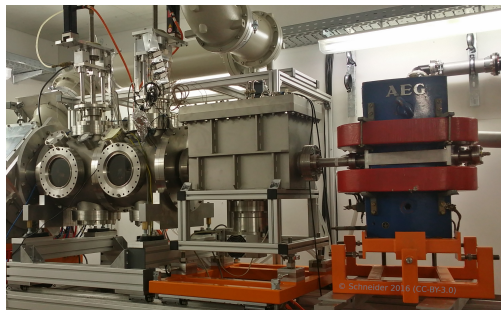
Figure 1: The diagnostic train in operation (left to right): emittance meter – beam dump – momentum spectrometer.
