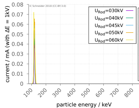
Figure 3: Energy histogram for a Helium beam (120 keV, 1 mA) at various rod voltages of the RFQ in transport mode. The beam remains unaccelerated and the energy spread is very narrow. This makes it perfect for the calibration of a momentum spectrometer.
