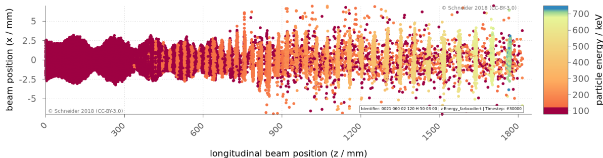
Figure 4: z - x -plane of the RFQ in acceleration mode, the energy of the individual particles is color-coded. The final energy is 700 keV (green), which is reached in the last cell. Parameters are: U_{\text{Rod}} = 60 kV, I_{\text{Beam}} = 50 mA, W_{\text{B,in}} = 120 keV.
