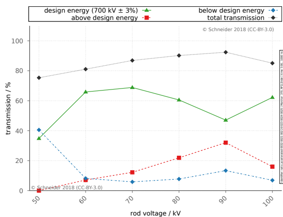
Figure 5: Influence of the rod voltage on the transmission of a proton beam (120 keV, 50 mA) at rod voltages of U_{\text{Rod}} = 50 kV...100 kV operating the RFQ in acceleration mode. It can be seen that the optimal transmission does not necessarily coincide with the largest proportion of accelerated particles.
