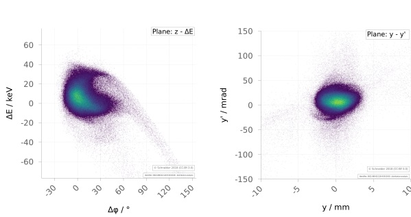
Figure 8: Particle distributions for the simulation of 50 mA protons with W_B = 700 keV at a rod voltage of 60 kV.
