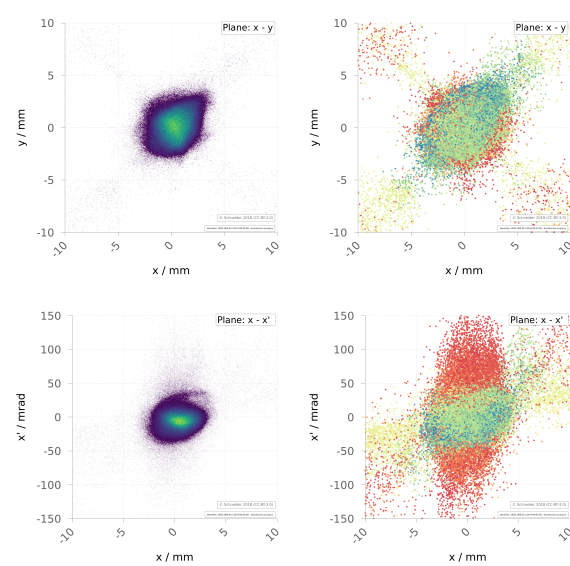
Figure 9: Particle distributions of the simulation of 50 mA protons with W_B = 700 keV at a rod voltage of 60 kV.
