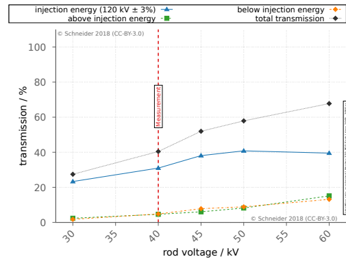
Figure 2: Influence of the rod voltage on the transmission of a Helium beam (120 keV, 1 mA) at rod voltages of U_{Rod} = 30\text{ kV} \dots 60\text{ kV} , operating the RFQ in transport mode. The beam remains unaccelerated. The measurements of [2] were performed at U_{Rod} \approx 40\text{ kV} .
