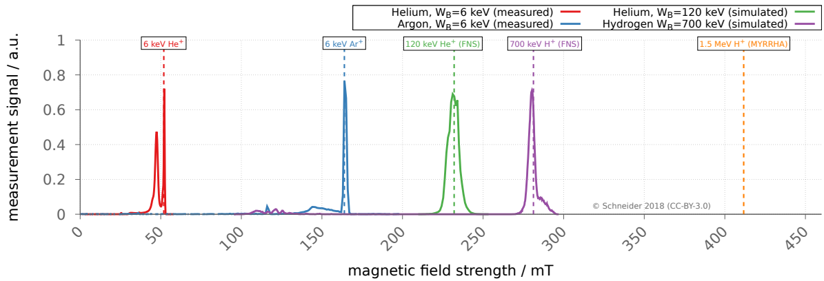
Figure 7: Momentum spectra of the several cases discussed in this paper. While Helium and Argon at W_B = 6 keV are measured, Helium at W_B = 120 keV and protons at W_B = 700 keV (both downstream the RFQ) are simulated with the PIC-code bender.
