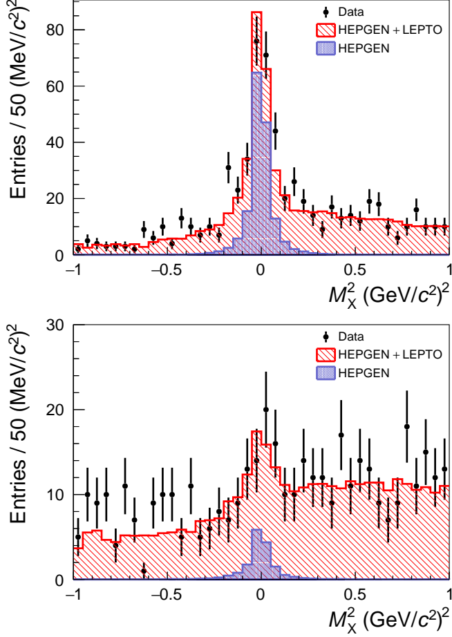
Figure 4: Distributions of the undetected mass M_X^2 for the signal (top) and background (bottom) reference samples, which are selected as described in Sect. 3 in the extended kinematic range Q^2 > 1(\text{GeV}/c)^2 , y > 0.05 and |t_{\text{TOF}}| > 0.08(\text{GeV}/c)^2 . Here, the quantities y and t_{\text{TOF}} denote the fractional energy loss of the muon and the squared four-momentum transfer to the recoil proton as measured by the target TOF system, respectively. Simulated data are also shown (see text). Note that events with the topology of exclusive \pi^0 production were removed from the LEPTO sample. Error bars denote statistical uncertainties.
