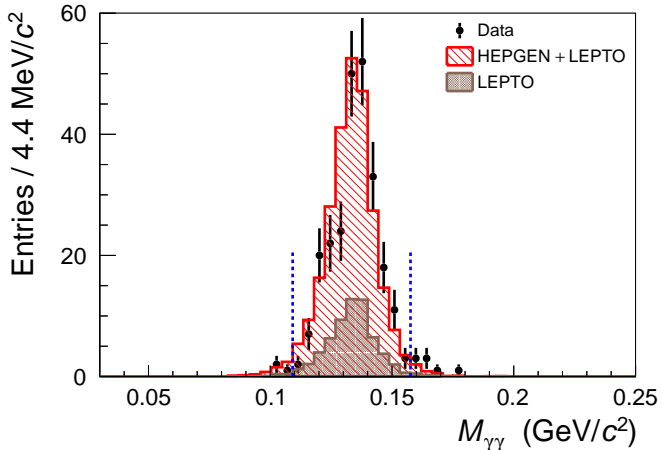
Figure 3: Distribution of the invariant mass M_{\gamma\gamma} of the two-photon system. Otherwise as in figure 2.
