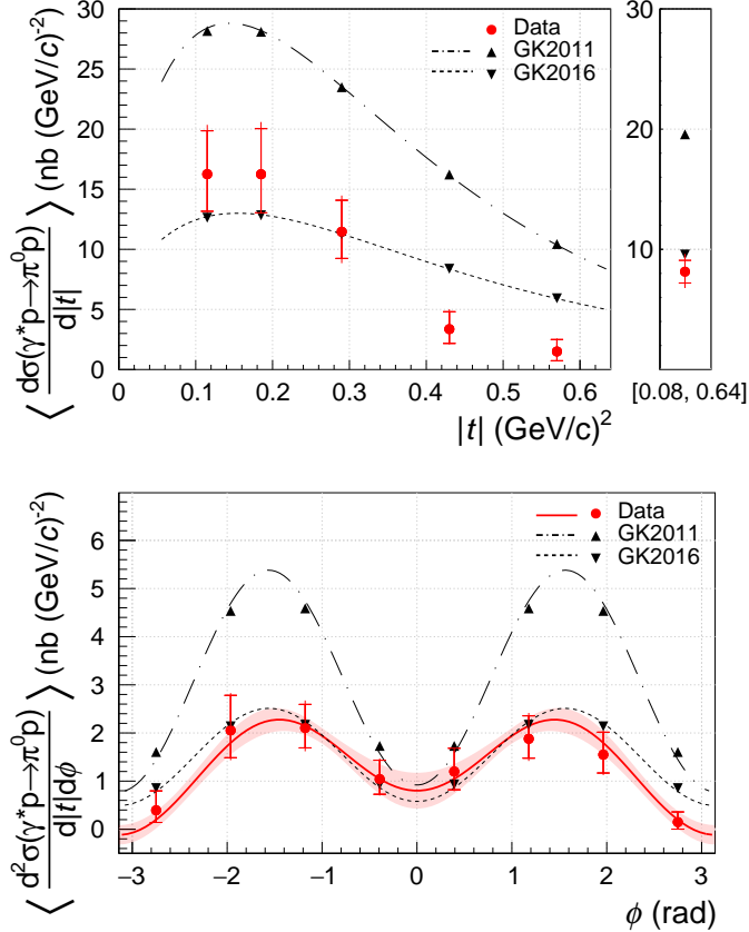
Figure 5: Average value of the differential virtual-photon proton cross section \langle \frac{d\sigma}{d|t|} \rangle as a function of |t| (top) and \langle \frac{d^2\sigma}{d|t|d\phi} \rangle as a function of \phi (bottom). For the top panel the data was integrated over \phi , while for the bottom panel it was integrated over |t| . The result of an integration over \phi and |t| is shown in the right-most part of the top panel. Inner error bars indicate the statistical uncertainty, outer error bars the quadratic sum of statistical and systematic uncertainties. The data is compared with two predictions of the GK model [15, 28]. Radiative corrections are not applied but an estimate is included in the systematic uncertainties.
