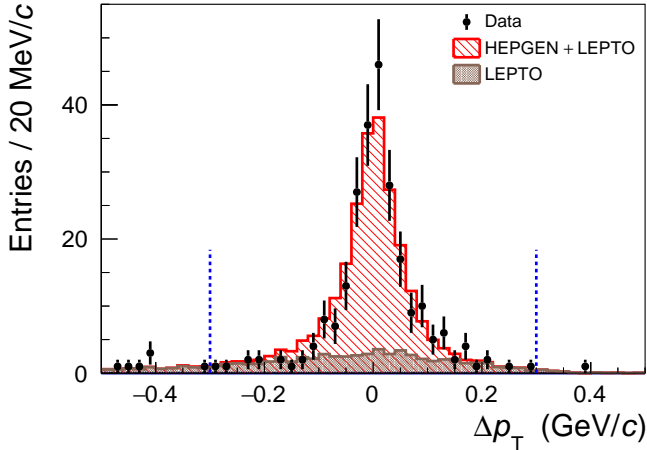
Figure 2: Measured and simulated distribution of the difference between predicted and reconstructed transverse momentum, \Delta p_T , of the recoil proton for the kinematic region described in the text. The vertical lines indicate the constraints applied for the selection of events. The quantity p_T is defined in the laboratory system. Error bars denote statistical uncertainties.
