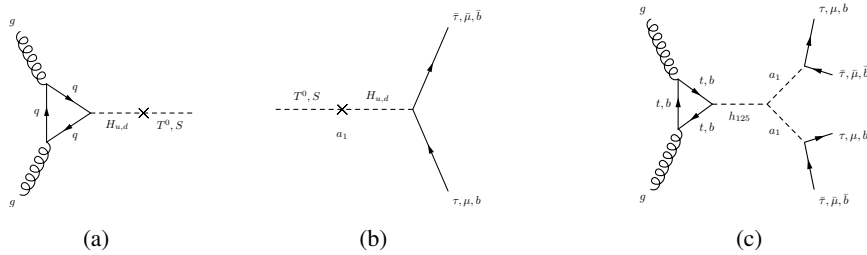
Figure 1: Feynman diagrams for the pair production of a singlet-like light pseudoscalar at the LHC.
