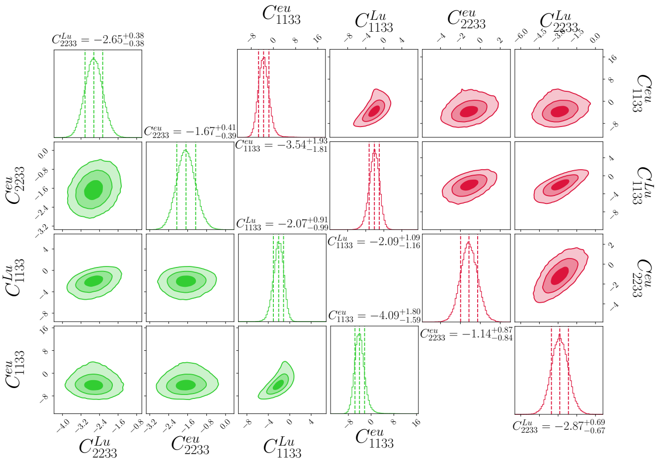
Fig. 10 Global fit of RGE-induced contributions ( \Lambda = 1 TeV) from eq. (17) constrained by b \rightarrow s\ell^+\ell^- data within the PMD (green) and PDD (red) approach, including the new R_K measurement. 16-th, 50-th, 84-th percentile for marginalized distributions is shown.
