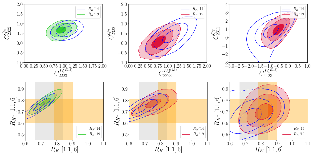
Fig. 4 2D p.d.f. for the scenario with WCs ( C_9^{NP}, C_{10}^{NP} ) and combined 2D p.d.f. of the corresponding results for R_K and R_{K^*} in both the PMD and the PDD approaches, following the colour scheme defined below fig. 2. We show the result in the SM gauge-invariant language, for both the muonic (left and central column) and electronic (right column) case.
