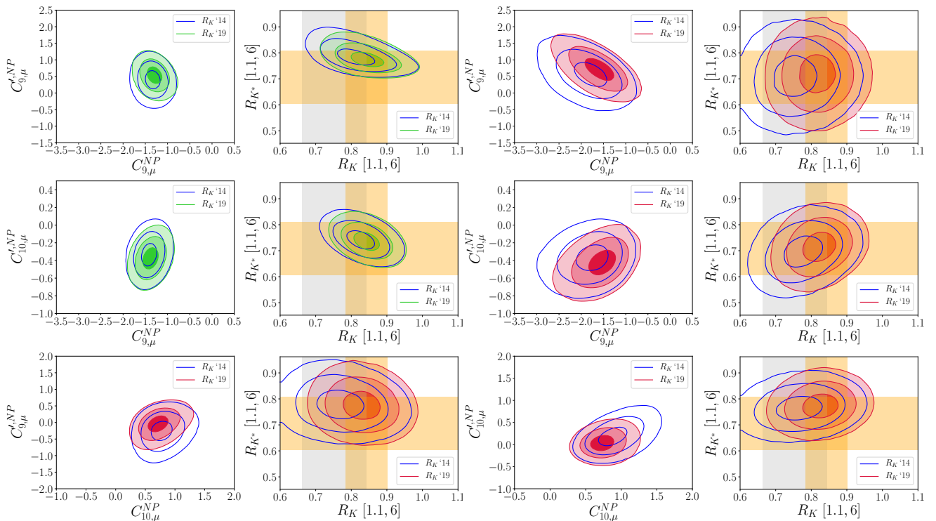
Fig. 5 First row: 2D p.d.f. for the scenario with WCs ( C_{9,\mu}^{\text{NP}}, C'_{9,\mu}{}^{\text{NP}} ) and combined 2D p.d.f. of the corresponding results for R_K and R_{K^*} in both the PMD and the PDD approaches, following the colour scheme defined below fig. 2. Second row: analogous to the first row, but relative to the WCs ( C_{9,\mu}^{\text{NP}}, C'_{10,\mu}{}^{\text{NP}} ). Third row: analogous to the first row, but in the PDD approach only and relative to the WCs ( C_{10,\mu}^{\text{NP}}, C'_{9,\mu}{}^{\text{NP}} ) and ( C_{10,\mu}^{\text{NP}}, C'_{10,\mu}{}^{\text{NP}} ).
