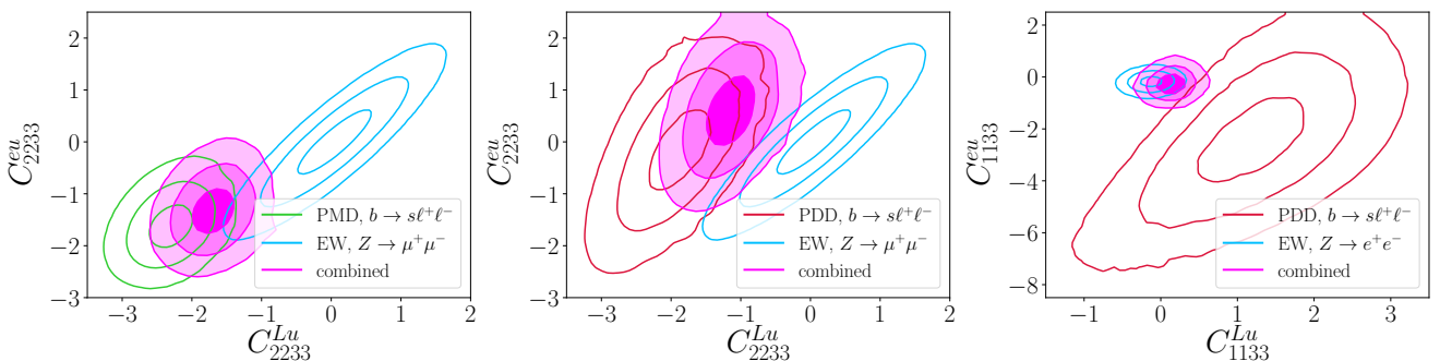
Fig. 11 2D p.d.f. for the scenario with WCs ( C_{\ell\ell 33}^{Lu} , C_{\ell\ell 33}^{eu} ) in both the PMD and the PDD approach, following the colour scheme defined below fig. 2. EW constraints on these scenario from Z \rightarrow \ell^+\ell^- measurements [207] are shown in light blue. The resulting region obtained from the combined information of EW and b \rightarrow s\ell^+\ell^- data is highlighted in fuchsia.
