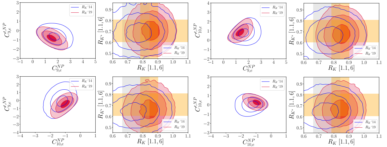
Fig. 6 First row: the first two panels show 2D p.d.f. for the scenario with WCs ( C_{9,e}^{\text{NP}}, C'_{9,e}{}^{\text{NP}} ) and the combined 2D p.d.f. of the corresponding results for R_K and R_{K^*} in the PDD approaches, following the colour scheme defined below fig. 2, while the last two panels show the same for the scenario with WCs ( C_{9,e}^{\text{NP}}, C'_{10,e}{}^{\text{NP}} ). Second row: analogous to the first row, but relative to the WCs ( C_{10,e}^{\text{NP}}, C'_{9,e}{}^{\text{NP}} ) and ( C_{10,e}^{\text{NP}}, C'_{10,e}{}^{\text{NP}} ).
