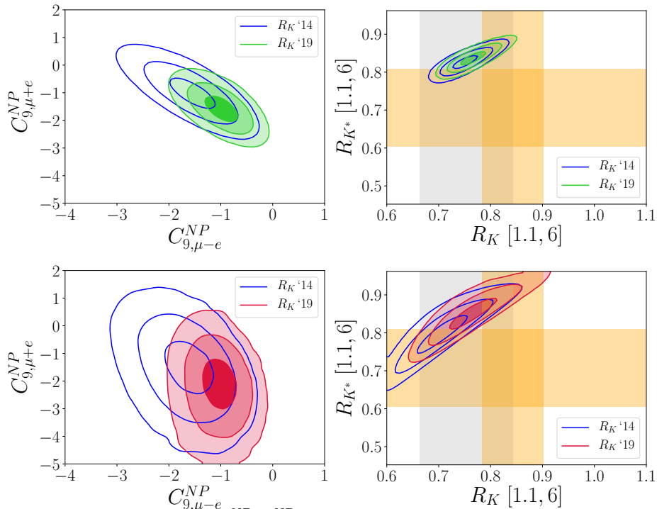
Fig. 3 2D p.d.f. for the scenario with WCs ( C_{9,\mu}^{NP}, C_{9,e}^{NP} ) and combined 2D p.d.f. of the corresponding results for R_K and R_{K^*} in both the PMD and the PDD approaches, following the colour scheme defined below fig. 2. In order to highlight the role of LFUV observables in this scenario we show in the left panels the WCs in the \mu \pm e combination.
