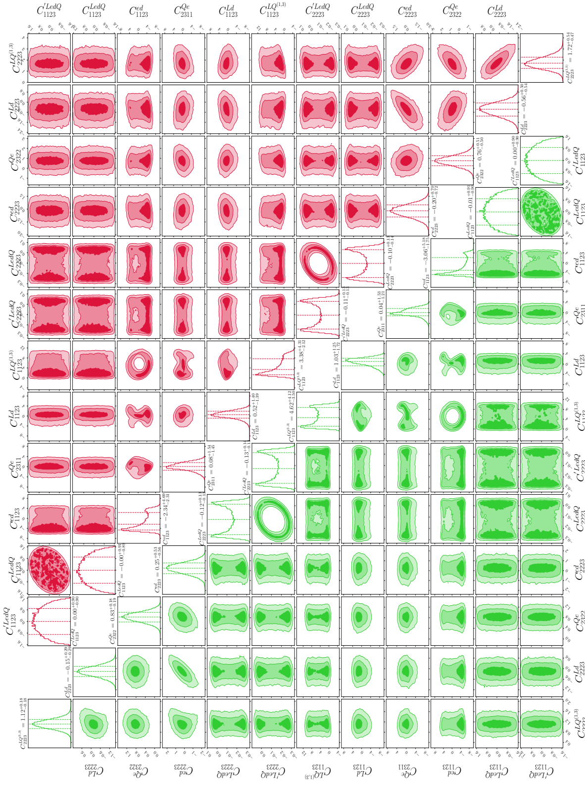
Fig. 9 Global fit of all tree-level SMEFT WCs ( \Lambda = 30 TeV) constrained by b \rightarrow s\ell^+\ell^- measurements within the PMD (green) and PDD (red) approach, including the 2019 R_K measurement. 16-th, 50-th, 84-th percentile for marginalized distributions is reported.
