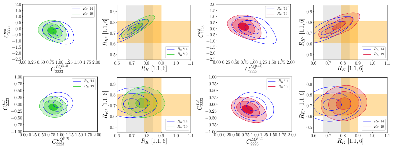
Fig. 7 First row: 2D p.d.f. for the scenario with WCs ( C_{2223}^{LQ(1,3)}, C_{2223}^{ed} ) and combined 2D p.d.f. of the corresponding results for R_K and R_{K^*} in both the PMD and the PDD approaches, following the colour scheme defined below fig. 2. Second row: analogous to the first row, but relative to the WCs ( C_{2223}^{LQ}, C_{2223}^{Ld} ).
