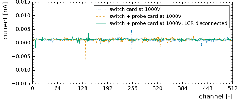
Figure 4: The system's leakage current per channel at 1000 V.
