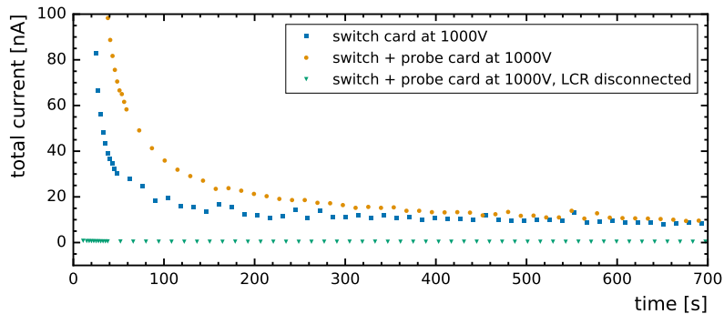
Figure 3: The system's total current over time at 1000 V.
