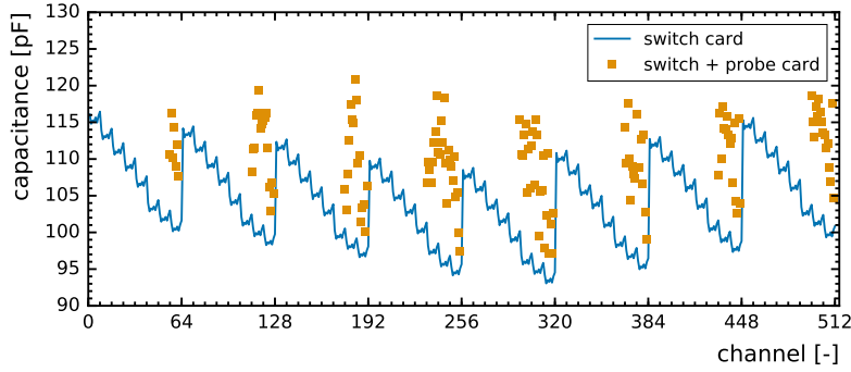
Figure 5: The capacitance per channel for the switch card with and without a 136 channel probe card connected. In the latter case, only the connected channels are measured. The measured values are then subtracted from consequent sensor measurements.
