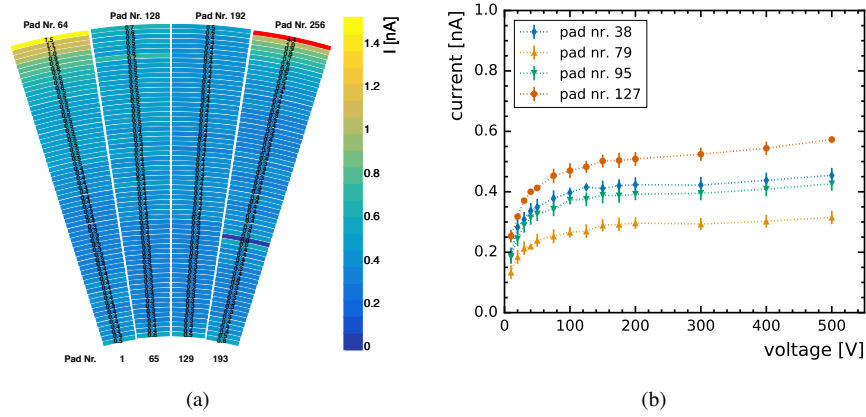
Figure 6: (a) Leakage current map of a LumiCal prototype sensor at 500 V bias (colour on-line). The current of one badly contacted pad is distributed to neighbouring pads. (b) Example IV curves from the same sensor. The error bars corresponds to the standard deviation from five consecutive measurements.
