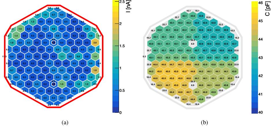
Figure 7: Pad values for (a) leakage current at 1000 V and (b) capacitance at 400 V measured with 1 kHz for an example 6-inch 135 pad p-on-n sensor measured with the ARRAY system (colour on-line). The four quadrants in the capacitance measurements correspond to four different cell geometries on the sensor. The guard ring is depicted as a line surrounding the sensor pads.
