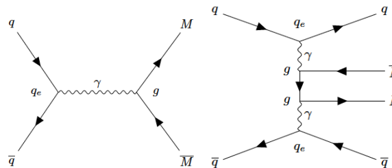
FIG. 4. Feynman-like diagrams for monopole pair direct production at leading order via the Drell-Yan (left) and photon fusion (right) processes at the LHC. For scalar and vector monopoles a four-vertex diagram is also added [30].
