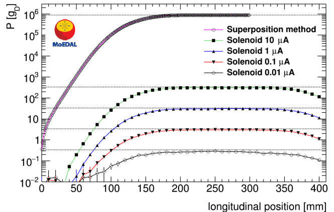
FIG. 1. Results of the calibration measurements with the superposition method using a magnetic dipole sample, and the solenoid method with P = 32.4g_{\text{D}}/\mu\text{A} and various currents. The dashed lines represent the expected plateau values in units of Dirac charge. The calibration constant is tuned using the measurement from the superposition method.
